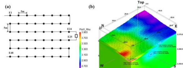
Fig. 1: 3D-ERT method (a) Electrode layout, (b) Location of Anomaly.
