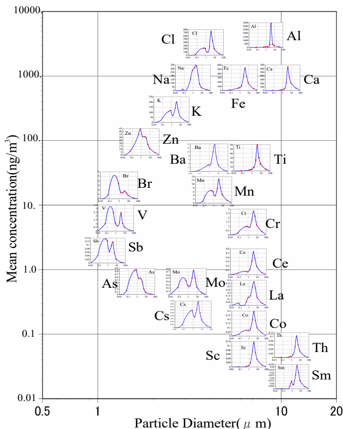
Fig.1 Size distributions of element in the atmospheric aerosols observed at Sakai,Osaka. Each size distribution is located at the position made by mean concentration and mean size for each element.
