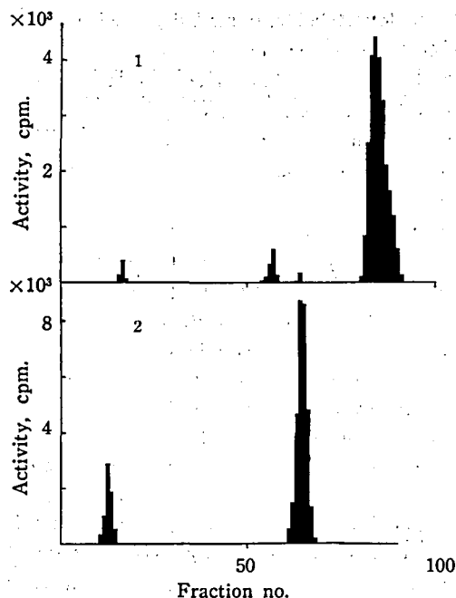
Fig. 3 Degradation products from methyl parathion and methyl paraoxon following incubation with supernatant of rat liver homogenate under anaerobic condition.
