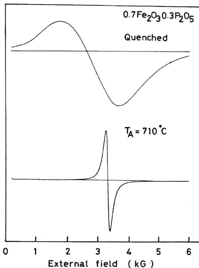
Fig.6.2 ESR spectra of 70\text{Fe}_2\text{O}_3 \cdot 30\text{P}_2\text{O}_5 quenched glass and heat-treated at 710^\circ\text{C} . T_A means the heat treatment temperature.
