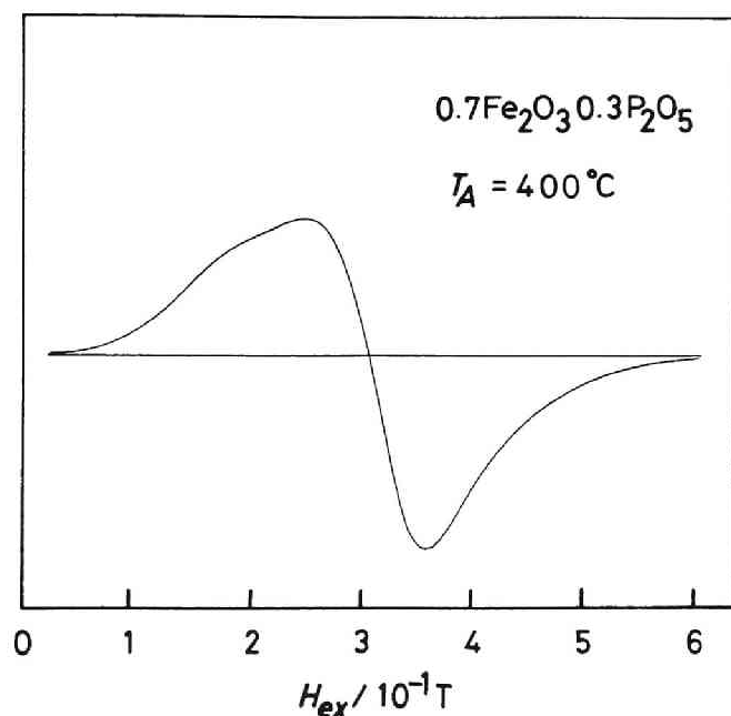
Fig.6.5 ESR spectrum of 70Fe 2 O 3 ·30P 2 O 5 glass heat-treated at 400 °C
