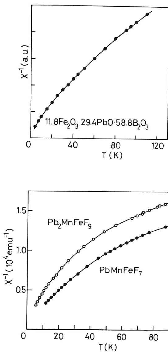
Fig.3.6 The temperature dependence of the susceptibility for several oxide and fluoride glasses. The inverse susceptibility vs. temperature curve in the superparamagnetic region shows the downward curvature.
