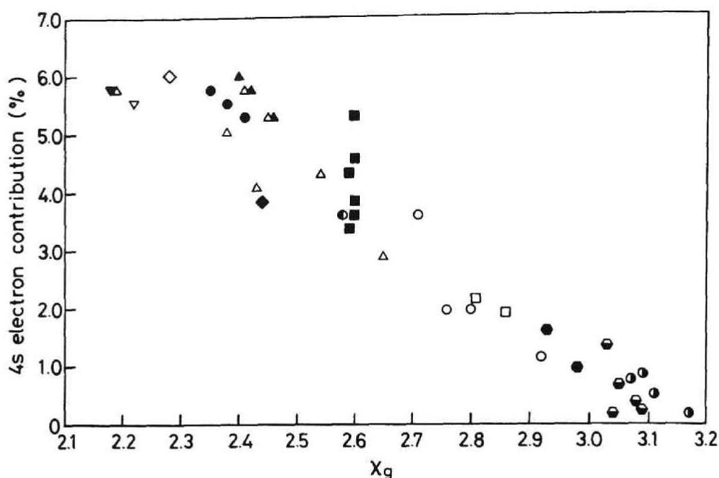
Fig.4.10 Relation between 4s electron contribution and the electronegativity \chi_g for several oxide and fluoride glasses. ○: \text{Fe}_2\text{O}_3\text{-P}_2\text{O}_5 , □: \text{Fe}_2\text{O}_3\text{-TeO}_2 , ■: \text{Fe}_2\text{O}_3\text{-Bi}_2\text{O}_3 , ▲: \text{Fe}_2\text{O}_3\text{-PbO} , ●: \text{Fe}_2\text{O}_3\text{-SrO} , ◇: \text{Fe}_2\text{O}_3\text{-BaO} , ◆: \text{Fe}_2\text{O}_3\text{-Y}_2\text{O}_3 , ▽: \text{Fe}_2\text{O}_3\text{-Na}_2\text{O} , ▼: \text{Fe}_2\text{O}_3\text{-K}_2\text{O} , △: \text{Fe}_2\text{O}_3\text{-Na}_2\text{O-B}_2\text{O}_3 , ●: \text{Fe}_2\text{O}_3 , ⦿: \text{FeF}_3\text{-PbF}_2\text{-MnF}_2 , ⦿: \text{FeF}_3\text{-BaF}_2\text{-ZrF}_4 , ⦿: \text{FeF}_3\text{-BaF}_2\text{-RF}_2 (R: Pb, Zn)
