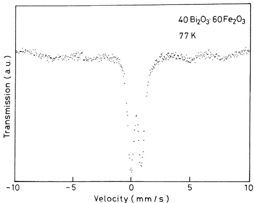
Fig.4.18 Mössbauer spectrum of 40\text{Bi}_2\text{O}_3 \cdot 60\text{Fe}_2\text{O}_3 glass at 77 K.
