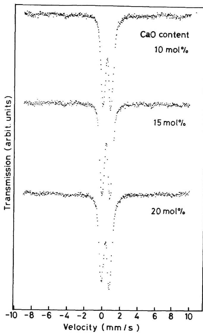
Fig.3.8 Mössbauer spectra of amorphous 10\text{CaO} \cdot 30\text{Bi}_2\text{O}_3 \cdot 60\text{Fe}_2\text{O}_3 , 15\text{CaO} \cdot 25\text{Bi}_2\text{O}_3 \cdot 60\text{Fe}_2\text{O}_3 and 20\text{CaO} \cdot 20\text{Bi}_2\text{O}_3 \cdot 60\text{Fe}_2\text{O}_3 at room temperature.
