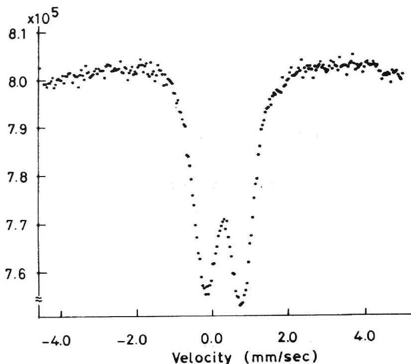
Fig.4.7 Mössbauer spectrum of 30\text{Na}_2\text{O} \cdot 40\text{Fe}_2\text{O}_3 \cdot 30\text{B}_2\text{O}_3 glass.
