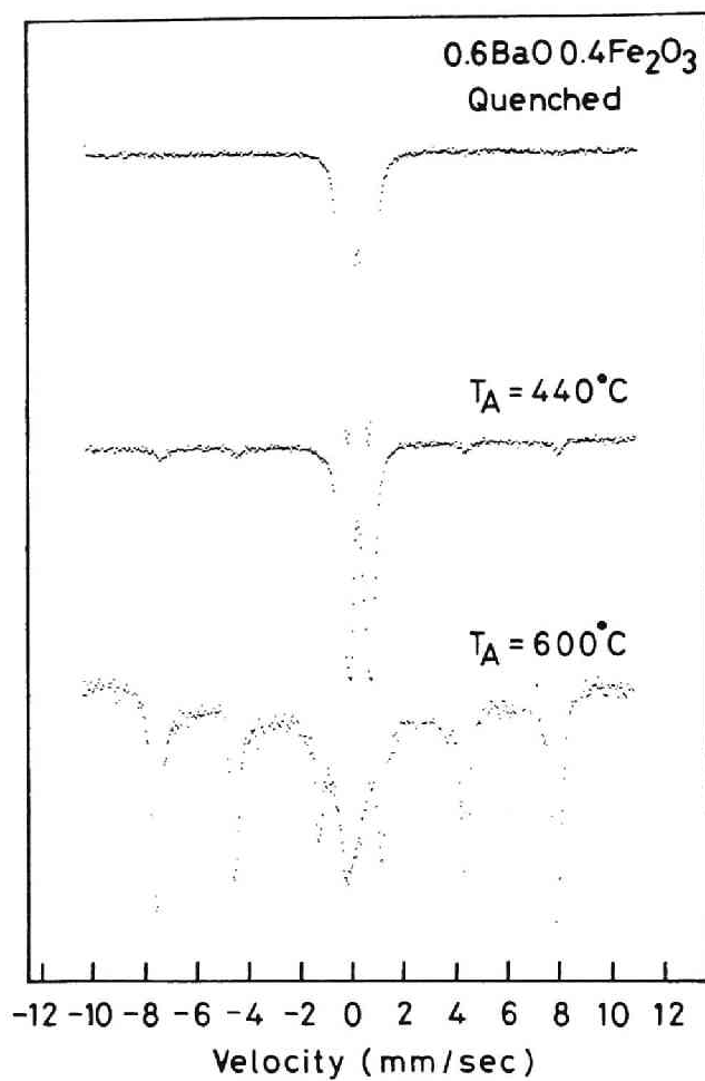
Fig.6.10 Mössbauer spectra of quenched, heat-treated at 440^\circ\text{C} and heat-treated at 600^\circ\text{C} 60\text{BaO} \cdot 40\text{Fe}_2\text{O}_3 glass. T_A means the heat treatment temperature.
