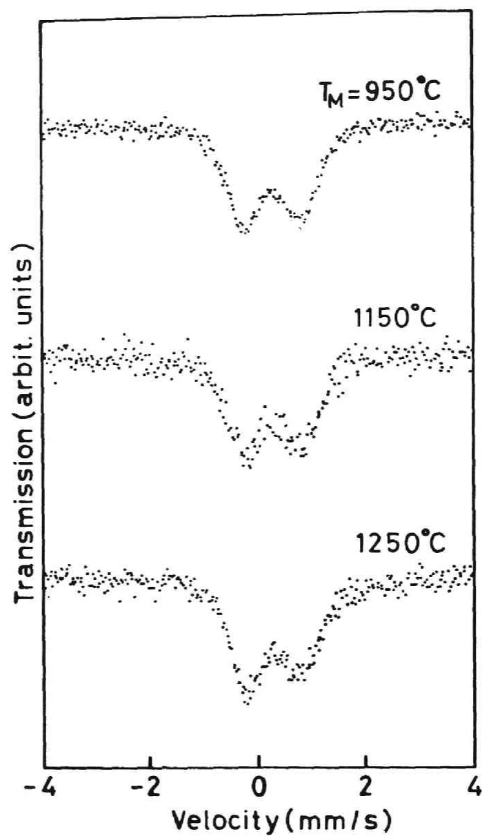
Fig.5.7 The Mössbauer spectra of \text{BaO} \cdot 2\text{B}_2\text{O}_3 glass containing 5 mol% \text{Fe}_2\text{O}_3 prepared by melting at several temperatures.
