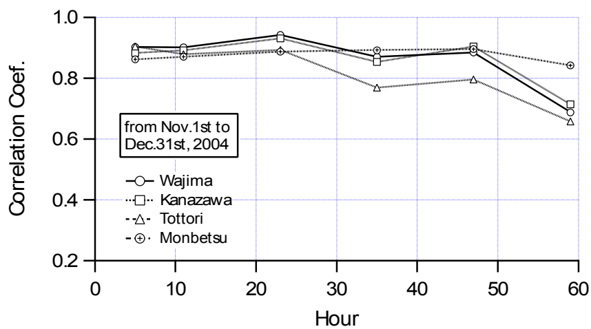
Fig. 3.20 GFS-SWAN correlation coefficient for winter
