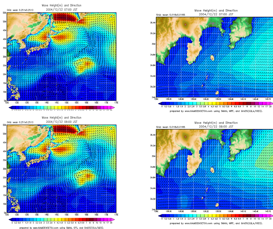
Fig. 3.5 Forecasted wave heights and directions for outer and nested domains
