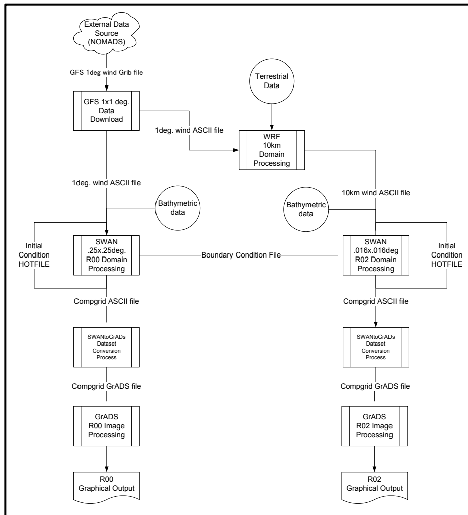
Fig. 3.2 Data flow diagram
