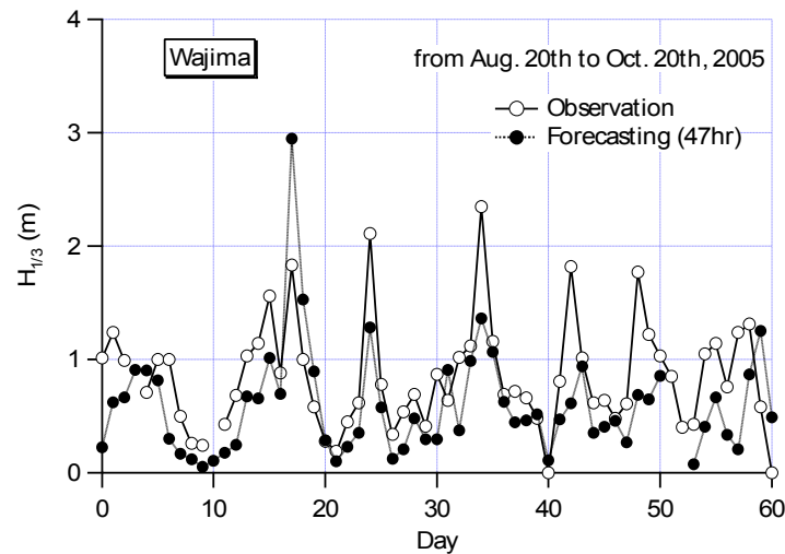
Fig. 3.16 GFS-SWAN significant wave height comparison for fall
