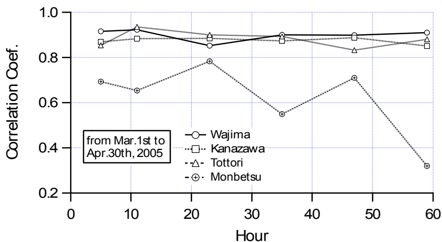
Fig. 3.18 GFS-SWAN correlation coefficient for spring
