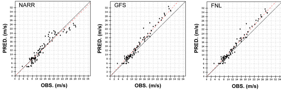
Fig. 4.8 Scatter plot of NARR, GFS and FNL wind speeds at NDBC station 42040
