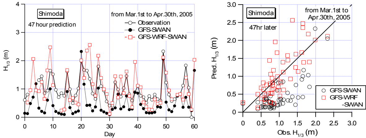
Fig. 3.21 Predicted and observed wave height comparison at Shimoda
