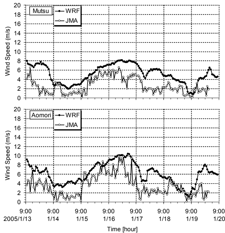
Fig. 3.14 GFS-WRF comparison for Mutsu and Aomori during winter
