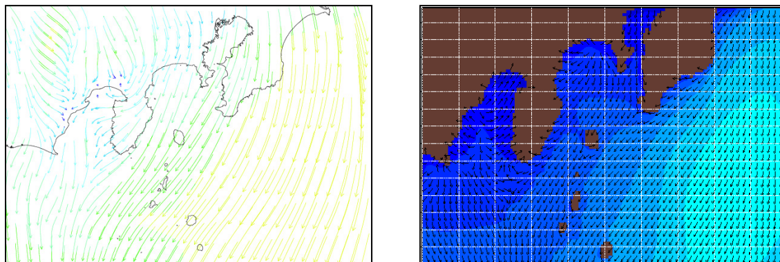
Fig. 3.4 WRF 10 km wind forecast (left) and resulting wave height and direction (right) for nested domain at 10/23/2004 00:00 GMT
