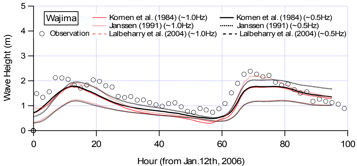
Fig. 3.23 Wave height calculation results using six different parameters
