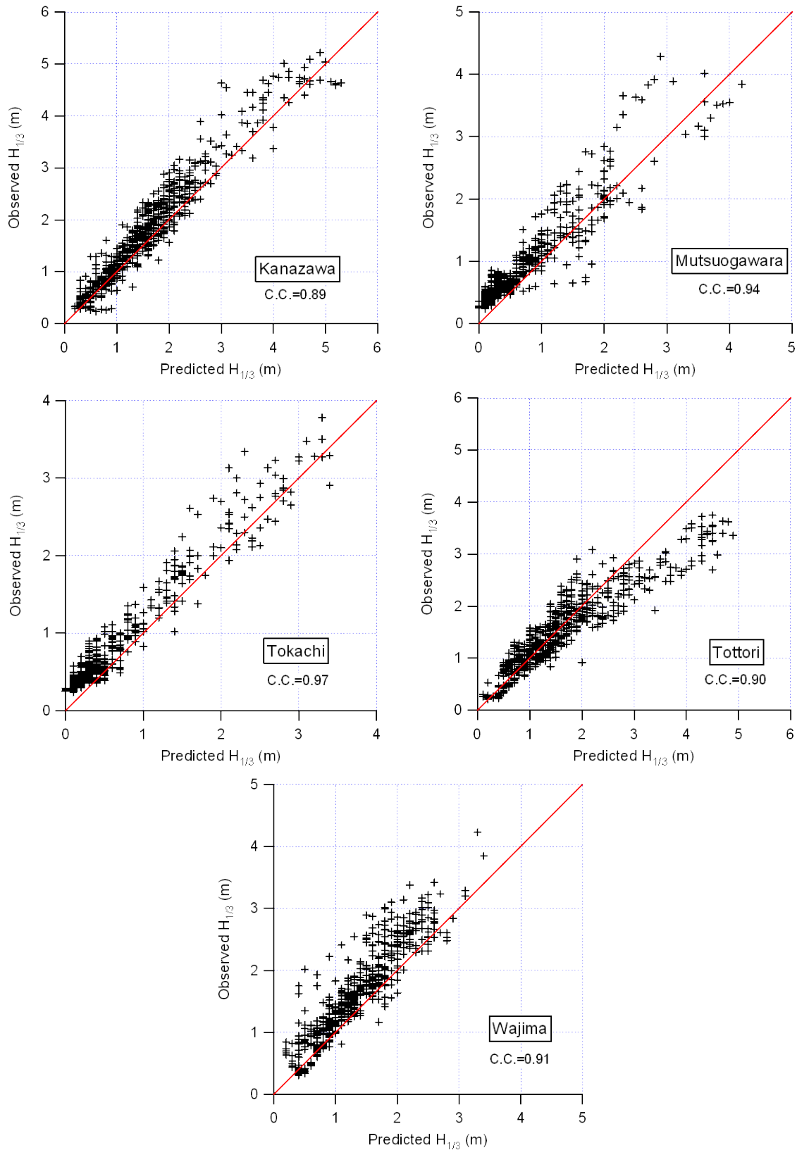
Fig. 5.6 Comparison of predicted vs. observed wave heights
