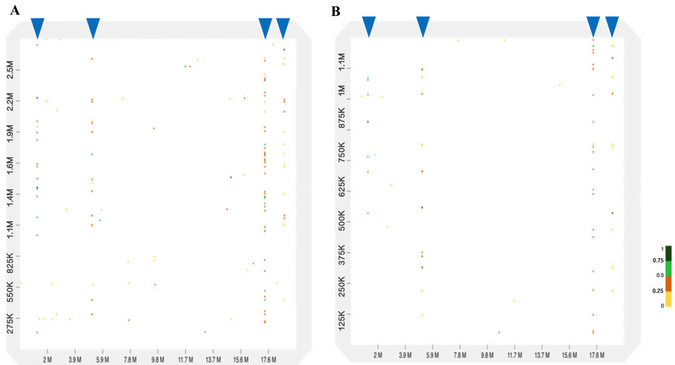
Figure 7. Dot plot analyses between chrW in Pyxicephalus adspersus and two scaffold sequences in Glandirana rugosa .
