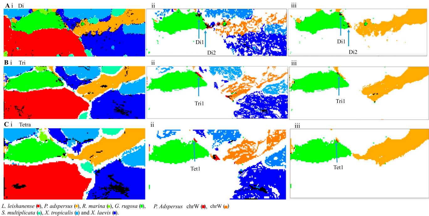
Figure 6. Batch-learning self-organizing maps (BLSOMs) for 1-Mb sequences sliding with a 10-kb step.
