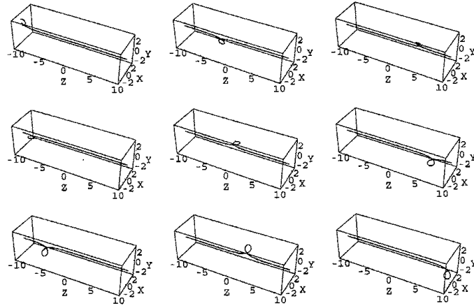
図 1: Loop soliton propagation v = 0.24, \Omega = 0.12
