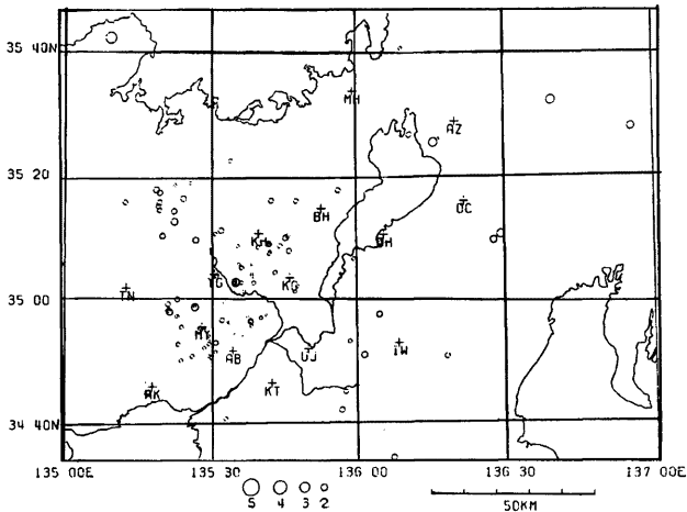
Fig. 9. Sismicity map around Lake Biwa in Sept. 1975.
