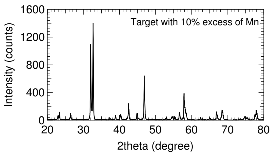
Figure 2.5: Powder XRD pattern for a sputtering target containing 10 % of Mn in excess.
