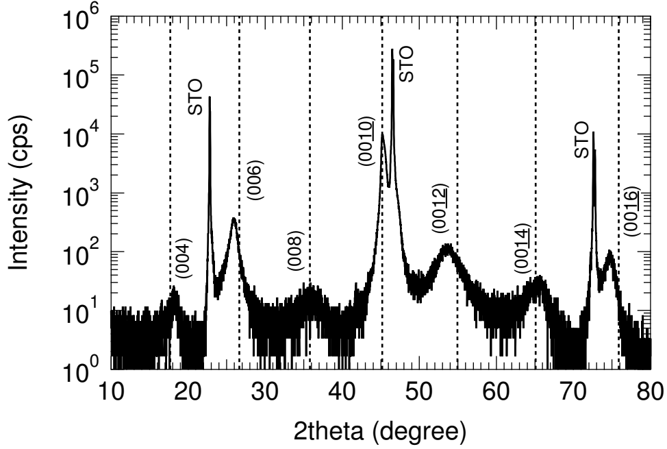
Figure 4.12: XRD pattern for a c -axis epitaxial layered manganate thin film, showing the shift of the XRD peaks from their positions calculated using the (00 10 ) peak (dotted lines).
