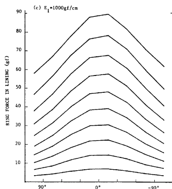
Fig. 11 Distribution of the ring force in lining.
