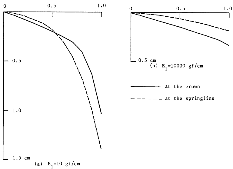
Fig. 15 Effect of lining rigidity on convergence of tunnel section.
