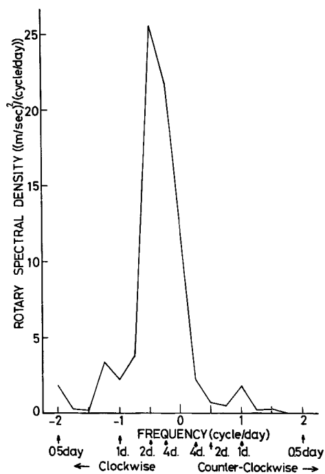
Fig. 14 The rotary spectrum of mean wind velocity vector.
