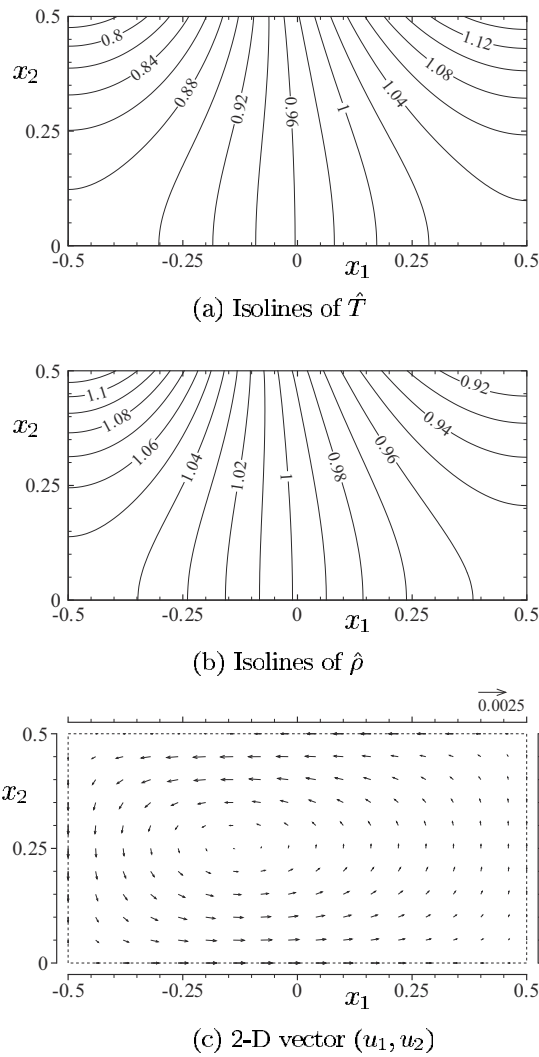
FIG. 2. Behavior of the free-molecular gas ( \text{Kn} \rightarrow \infty ) in the case of the Cercignani-Lampis model with (\alpha_n, \alpha_t) = (0.7, 0.5) . See the caption of Fig. 1.
