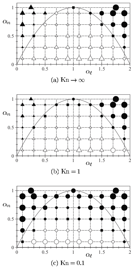
FIG. 6. Type of the flow field in the case of the Cercignani-Lampis model with various \alpha_n and \alpha_t . (a) \text{Kn} \rightarrow \infty , (b) \text{Kn}=1 , and (c) \text{Kn}=0.1 . Here, \triangle , \circ , \blacktriangle , and \bullet indicate the I-, II-, III-, and IV-type flows, respectively. The symbol size indicates the maximum flow speed U[\equiv \max(u_1^2 + u_2^2)^{1/2}] ; small symbols are used for 1 \times 10^{-3} \leq U < 8 \times 10^{-3} , middle symbols for 8 \times 10^{-3} \leq U < 1.6 \times 10^{-2} , and large symbols for U \geq 1.6 \times 10^{-2} . \blacksquare indicates the case where U < 1 \times 10^{-3} or the flow field is not classified into any of the four types. The solid line is the parabola \alpha_n = \alpha_t(2 - \alpha_t) .
