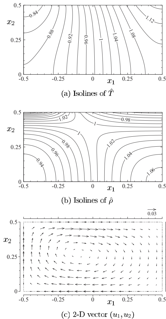
FIG. 4. Behavior of the free-molecular gas ( \text{Kn} \rightarrow \infty ) in the case of the Cercignani-Lampis model with (\alpha_n, \alpha_t) = (1, 1.75) . See the caption of Fig. 1.
