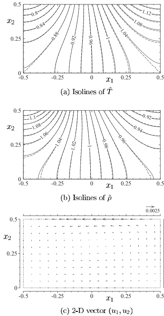
FIG. 8. Comparison of behavior of the free-molecular gas ( \text{Kn} \rightarrow \infty ) under the different boundary conditions. (a) Isolines of the (dimensionless) temperature \hat{T} , (b) those of the density \hat{\rho} , and (c) the flow velocity (u_1, u_2) . In panels (a) and (b), the solid lines indicate results of the Cercignani–Lampis model with (\alpha_n, \alpha_t) = (0.75, 0.5) and the dashed lines indicate those of the Lord model with \sigma = 0.75 . Panel (c) shows the results for the Cercignani–Lampis model.
