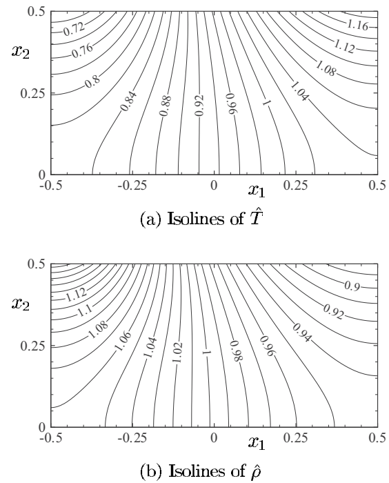
FIG. 5. Behavior of the free-molecular gas ( \text{Kn} \rightarrow \infty ) in the case of the Cercignani-Lampis model with (\alpha_n, \alpha_t) = (1, 1) , which is equivalent to the diffuse reflection. (a) Isolines of the (dimensionless) temperature \hat{T} and (b) those of the density \hat{\rho} .
