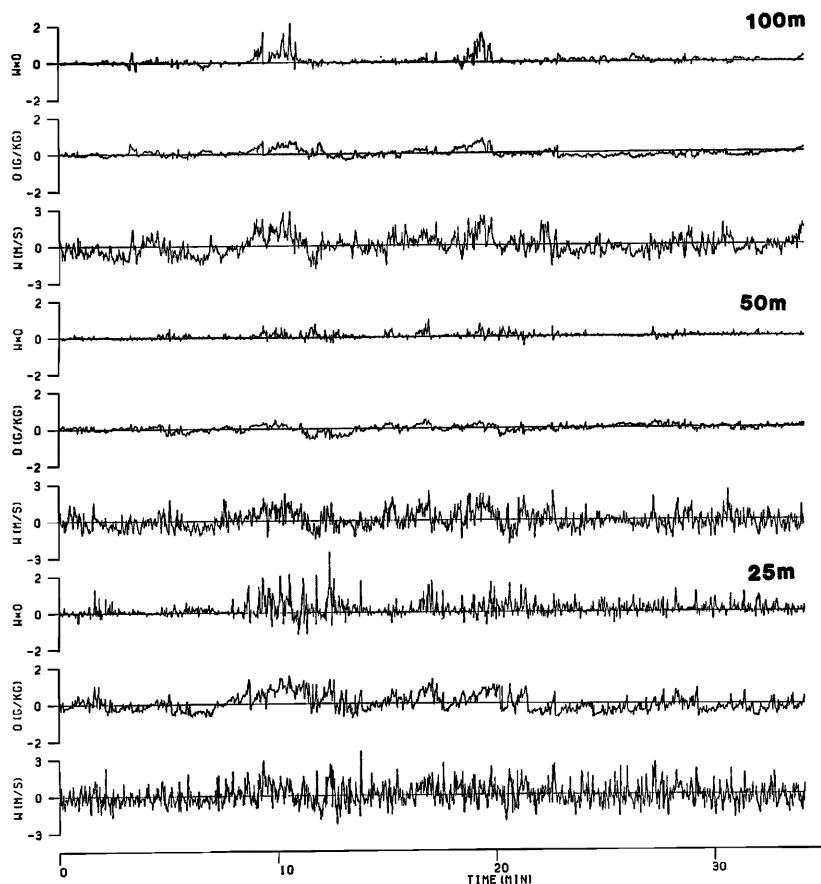
Fig. 2 An example of time histories of the cross product of vertical wind component and specific humidity fluctuation, and the fluctuations of both components for each level from the top to the bottom.
