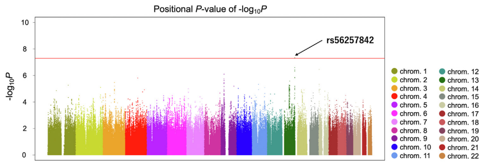
Figure 1. Manhattan plot of the genome-wide meta-analysis for myopic macular neovascularization (mMNV). Each plot shows -\log_{10} -transformed P values for all SNPs adjusted for age, sex, and axial length. The red horizontal line represents the genome-wide significance threshold ( P = 5.0 \times 10^{-8} ). rs56257842 at TEX29 - LINC02337 was genome-wide significantly associated with myopic macular neovascularization development (OR [95% CI] = 0.62 [0.52–0.73], P = 4.63 \times 10^{-8} ).
