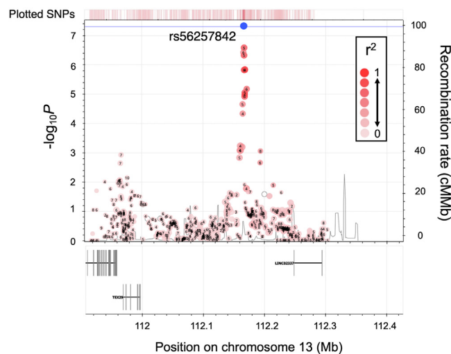
Figure 4. Regional association plots for genotyped single nucleotide polymorphisms (SNPs) around rs56257842 at TEX29 - LINC02337 . Plots represent the -\log_{10}(P) values obtained from the genome-wide meta-analysis for SNPs located within 500 000 base pairs of rs56257842. Association signals were observed extending upstream of LINC02337 .
