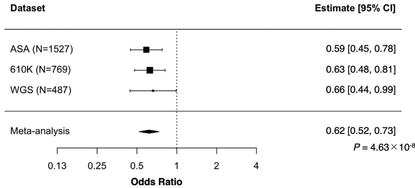
Figure 3. A forest plot depicting the effect of rs56257842 at TEX29 - LINC02337 on myopic macular neovascularization (mMNV). rs56257842 (effect allele: C) at TEX29 - LINC02337 showed a consistent effect size on mMNV development in all data sets ( I^2 = 0.00 ). The effect size of the single nucleotide polymorphism in each data set was 0.59 (95% confidence interval [CI], 0.45–0.78; P = 1.71 \times 10^{-4} ), 0.63 (95% CI, 0.48–0.81; P = 5.53 \times 10^{-4} ), and 0.66 (95% CI, 0.44–0.99; P = 4.38 \times 10^{-2} ) for the Asian Screening Array (ASA) data set, 610K data set, and whole genome sequencing (WGS) data set, respectively.
