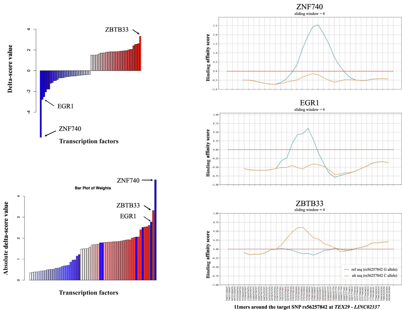
Figure 7. Impact of transcription factor (TF) binding to rs56257842 at TEX29 - LINC02337 . A , Bar plot of delta-scores for TFs that are ranked within the each top 30 for positive and negative delta-scores. TFs with positive delta-scores are presented in red and those with negative delta-scores are presented in blue. B , Bar plot of absolute delta-scores for TFs presented in (A). The binding affinity score is presented as an absolute value. TFs with positive values are presented in red and those with negative values are in blue. C–E , Binding affinity scores (vertical axis) of 11mer TF binding motifs around the target SNP rs56257842 at TEX29 - LINC02337 (horizontal axis) using the machine learning–based prediction method large-scale gkm-SVM; positive scores (above the red dotted lines) indicate more probable binding: C , Impact of TF binding for ZNF740 to rs56257842. Around rs56257842 (sliding window = 4), the reference 11mers exceed the threshold of a positive value (red dotted line), whereas alternative 11mers do not. When rs56257842 is G (ref) allele, the maximum binding affinity score is 2.538, but when rs56257842 is C (alt) allele, the maximum binding affinity score is 0. This means that ZNF740 loses the binding affinity when switching to the alternative (C) allele. D , Impact of TF binding of EGR1 to rs56257842. Around rs56257842 (sliding window = 4), the reference 11mers exceed the threshold of a positive value (red dotted line), whereas alternative 11mers does not. When rs56257842 is G (ref) allele, the maximum binding affinity score is 0.608, but when rs56257842 is C (alt) allele, the maximum binding affinity score is less than 0. This means that EGR1 loses the binding affinity when switching to the alternative (C) allele. E , Impact of TF binding of ZBTB33 to rs56257842. Around rs56257842 (sliding window = 4), the alternative 11mers exceed the threshold of a positive value (red dotted line), whereas reference 11mers does not. When rs56257842 is C (alt) allele, the maximum binding affinity score is 0.609, but when rs56257842 is G (ref) allele, the maximum binding affinity score is less than 0. This means that ZBTB33 gains the binding affinity when switching to the alternative (C) allele.
