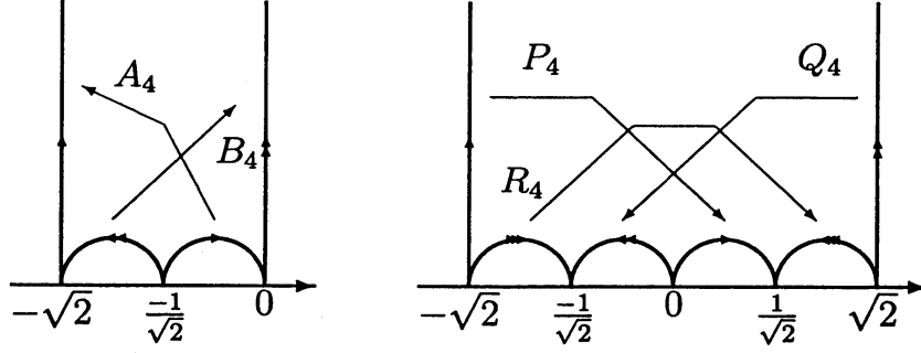
Figure 3: Fundamental domains of \Gamma_4^0 and \langle P_4, Q_4, R_4 \rangle .
