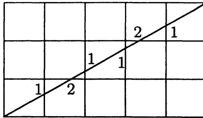
Figure 4: The cutting sequence of (5, 3) : 121121
