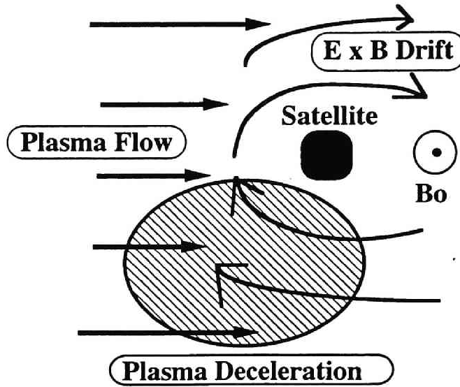
Figure 4.10: Schematic illustration showing the interaction between the ambient plasma flow and the E \times B drift.
