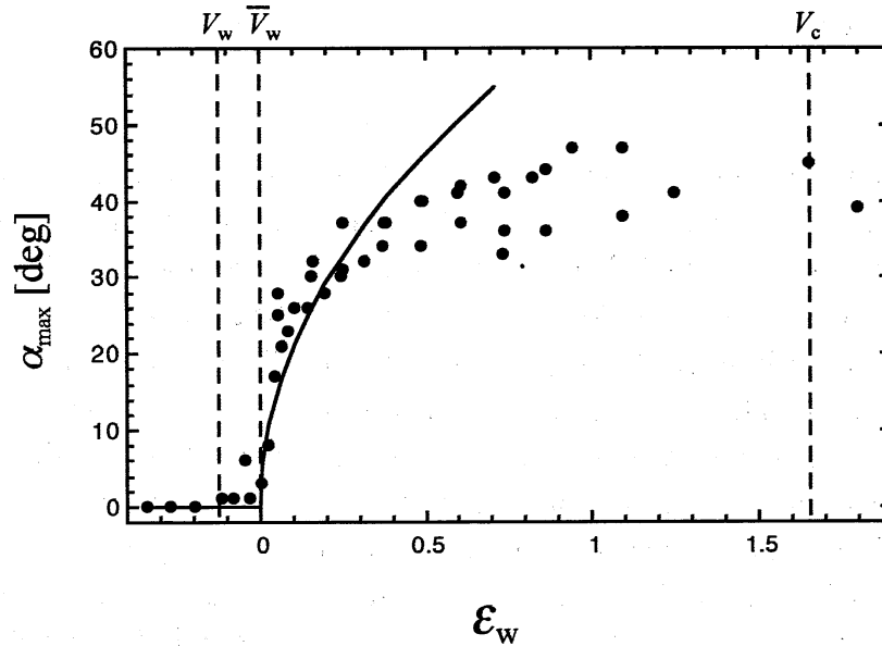
FIGURE 3 The in-plane rotation angle \alpha_{\max}(\varepsilon_w) (at f = 2150\text{Hz} ). The prewavy pattern becomes detectable at V_w . The thick lines correspond to a fit of \alpha_{\max}(\varepsilon_w) = \Phi \varepsilon_w^{1/2} . See the text for details.
