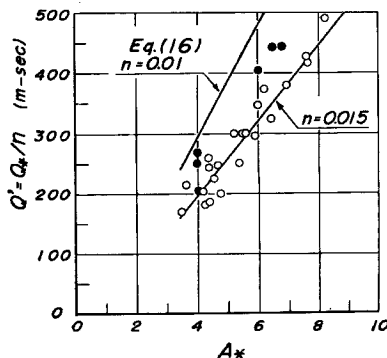
Fig. 15 Relationship between Q' and A_* for Stebbings' experiments.
