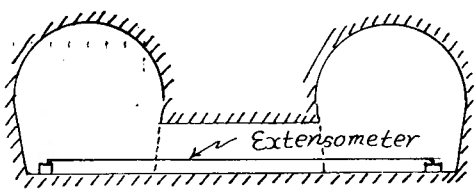
Fig. 3. Setting of extensometer C_1 in tunnels.
