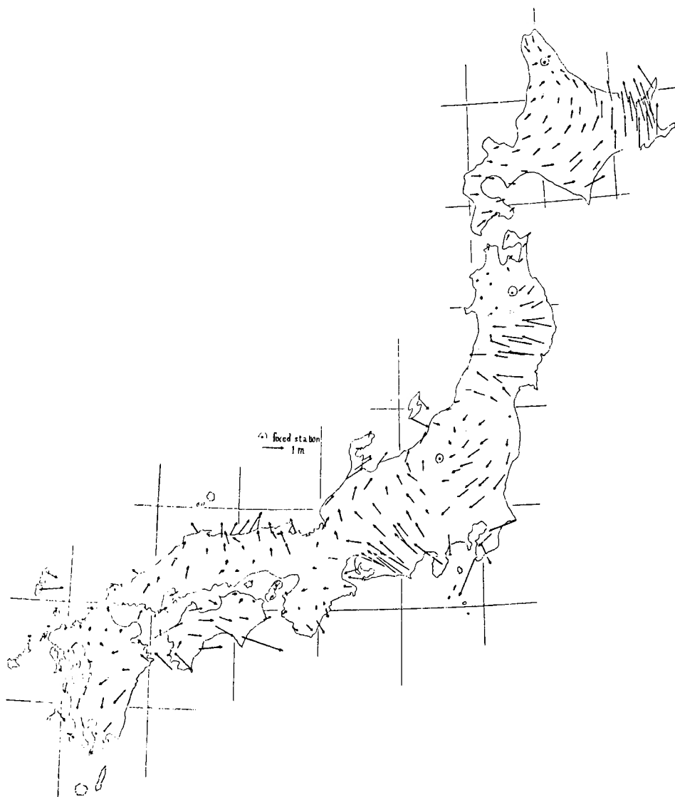
Fig. 4. Relative displacements of trianguration stations (After T. Harada).
