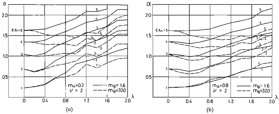
Fig. 10. Dimensionless intensity parameter \alpha for the response level E\gamma_{r,1} , (a) \nu=2 and m_0=0.2 , (b) \nu=2 and m_0=0.8 .
