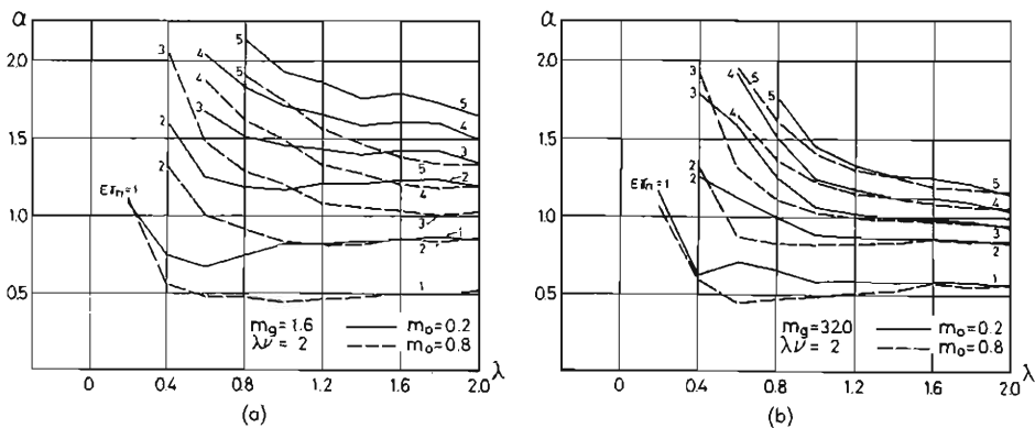
Fig. 11. Dimensionless intensity parameter \alpha for the response level E\gamma_{r,1} , (a) \lambda\nu=2 and m_g=1.6 , (b) \lambda\nu=2 and m_g=32.0 .
