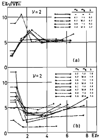
Fig. 8. Variation of EY_{r1}/\sqrt{V\gamma_{r1}} with E\gamma_{r1} .
