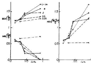
Fig. 13. Relation between D/h_1 and MAX\left(\frac{q_M}{\bar{q}}\right) , MIN\left(\frac{q_{70}}{\bar{q}}\right) and MAX\left(\frac{q_M - q_{70}}{\bar{q}}\right) .
