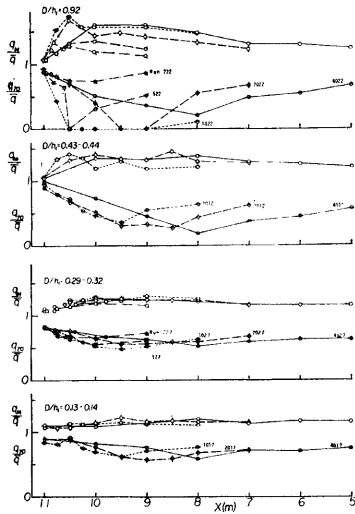
Fig. 12. Longitudinal variation of q_M/\bar{q} and q_{70}/\bar{q} .
