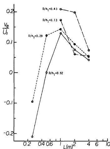
Fig. 16. Relation between v_e/U_1 and L .
