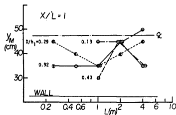
Fig. 11. The position of maximum discharge at the ends of abrupt drops.
