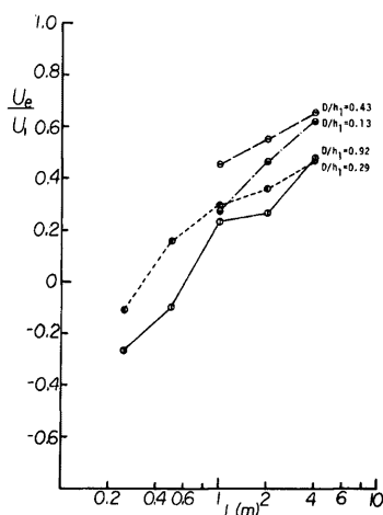
Fig. 15. Relation between U_e/U_1 and L .
