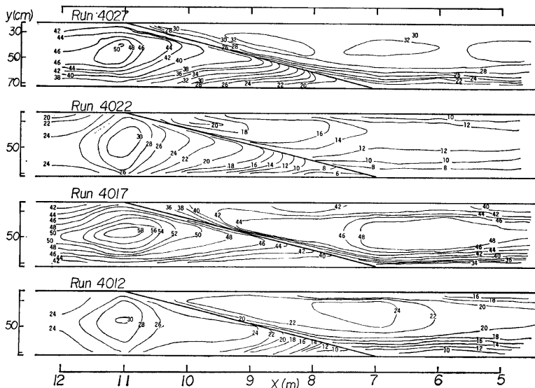
Fig. 4. Plane distribution of velocity near the channel bed ( L=4 m).
