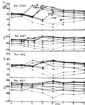
Fig. 9. Longitudinal variation of discharge per unit width.
