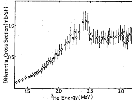
Fig. 4. The differential cross sections as a function of bombarding energy for the {}^9\text{Be}({}^3\text{He}, \alpha_1){}^8\text{Be} reaction at a laboratory angle of 165^\circ .
