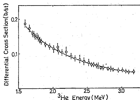
Fig. 2. The differential cross sections as a function of bombarding energy for the {}^9\text{Be}({}^3\text{He}, {}^3\text{He}){}^9\text{Be} reaction at a laboratory angle of 165^\circ .
