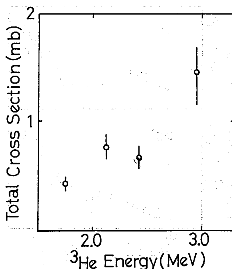
Fig. 6. The total cross sections as a function of bombarding energy for the ^9\text{Be}(^3\text{He}, \alpha_0)^8\text{Be} reaction.
