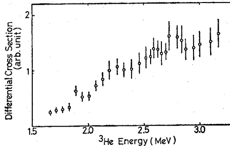
Fig. 5. The differential cross sections as a function of bombarding energy for the {}^9\text{Be}({}^3\text{He}, \alpha_3 + \alpha_4){}^8\text{Be} reaction at \theta_1 = 80^\circ and \theta_2 = -106^\circ .
