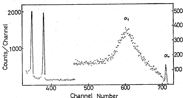
Fig. 1. Spectrum of alpha particles from the {}^9\text{Be}({}^3\text{He}, \alpha){}^8\text{Be} reaction at a bombarding energy of 2.007 MeV and a laboratory angle of 165^\circ .
