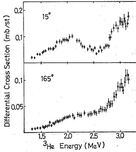
Fig. 3. The differential cross sections as a function of bombarding energy for the {}^9\text{Be}({}^3\text{He}, \alpha_0){}^8\text{Be} reaction at laboratory angles of 15^\circ and 165^\circ .
