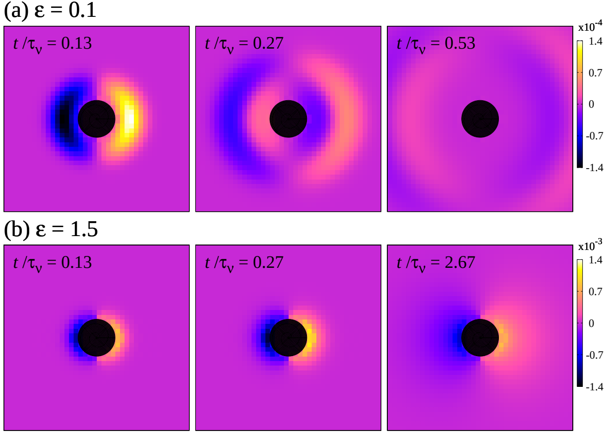
Figure 2.2: Time evolution of the fluid density deviation around the particle. The compressibility factors are (a) \varepsilon = 0.1 (upper row) and (b) \varepsilon = 1.5 (lower row). The color scale represents negative (darker) to positive (lighter) density deviation. The black circle represents the particle. The direction of the initial particle velocity is right in these pictures.
