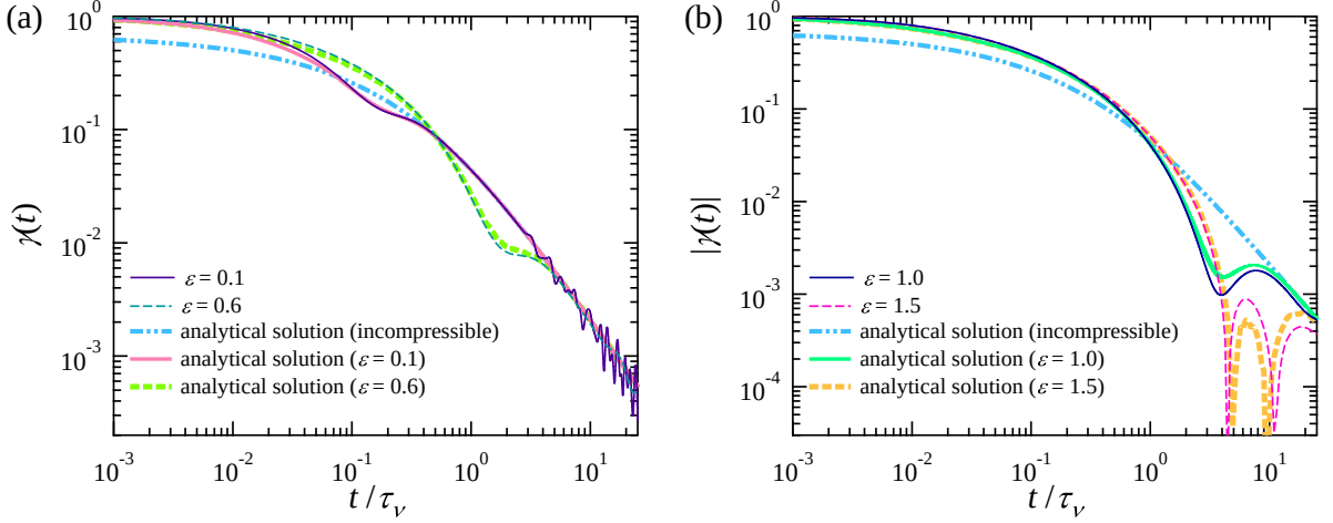
Figure 2.1: The velocity relaxation function for various compressibility factors: (a) \varepsilon = 0.1, 0.6 , (b) 1.0 , and 1.5 . The bold lines illustrate the analytic solutions for various compressibility factors, and the bold dashed double-dotted line shows the analytic solution for an incompressible fluid.
