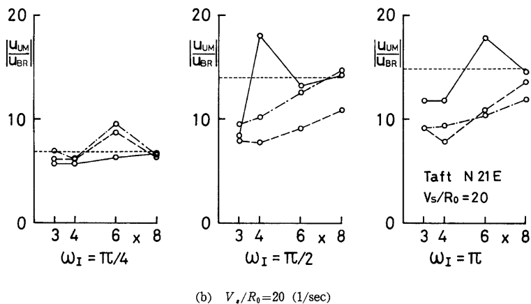
Fig. 20 Maximum responses of upper mass against separation distance, Taft N21E, d=2 , e=1 .
