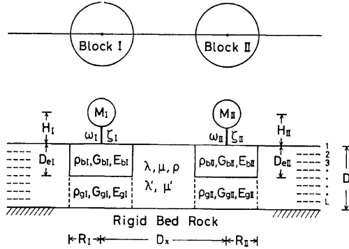
Fig. 3 Two-structures-soil system.
