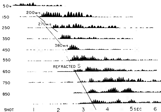
Fig. 2. Rectified wave forms of the horizontal component.
