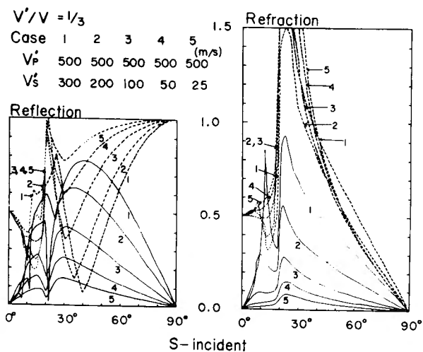
Fig. 11. Amplitudes of converted waves at the interface for incident S waves from lower medium.
