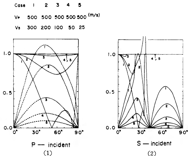
Fig. 12. Amplitudes of converted waves at the free surface.
