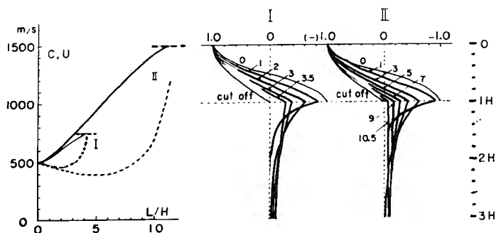
Fig. 7. Dispersion curves and amplitude distributions with depth to the P - P mode in liquid-liquid layers.
