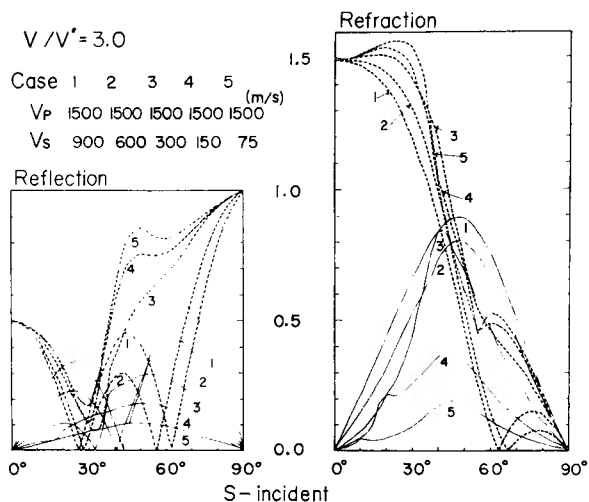
Fig. 10. Amplitudes of converted waves at the interface for incident S waves from upper medium.
