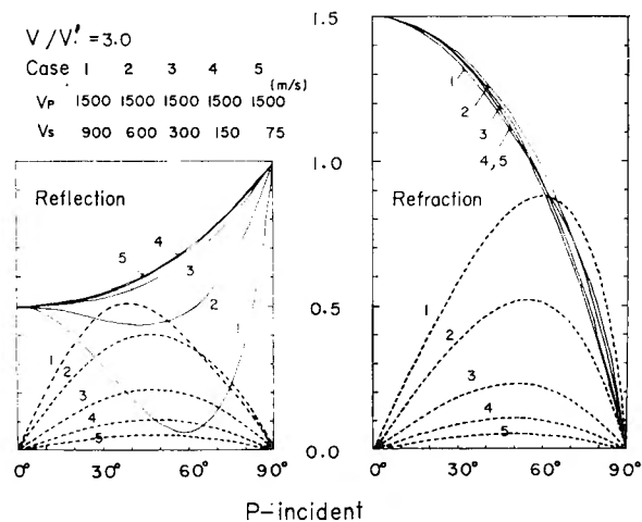
Fig. 8. Amplitudes of converted waves at the interface for incident P waves from lower medium.
