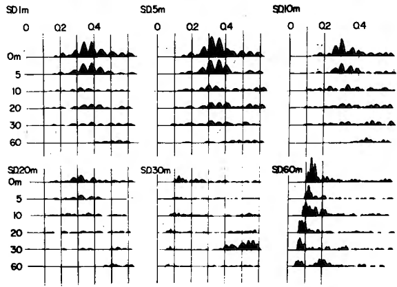
Fig. 4. Records from the various shot-depths.
