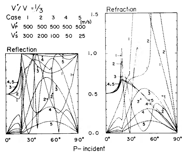
Fig. 9. Amplitudes of converted waves at the interface for incident P waves from upper medium.
