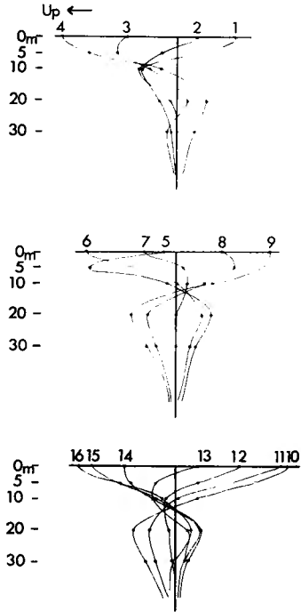
Fig. 6. Amplitude distributions with depth of the wave group II.
