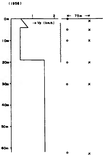
Fig. 3. Seismic profile, spreads of seismometers and shooting points of the experimental field at Sakata City in 1956.
