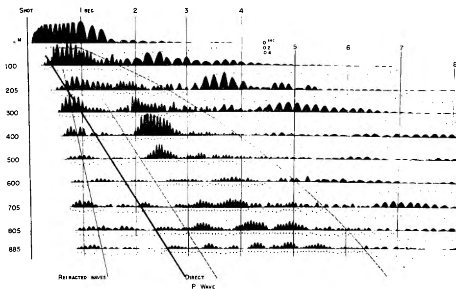
Fig. 1. Rectified wave forms of the vertical component.
