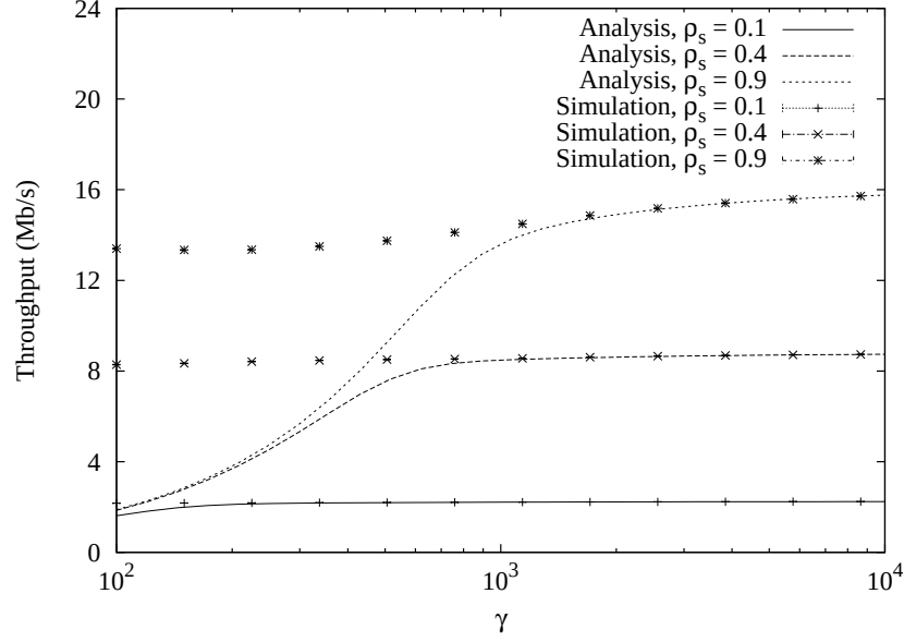
FIGURE 4. Throughput vs. sensing rate.
