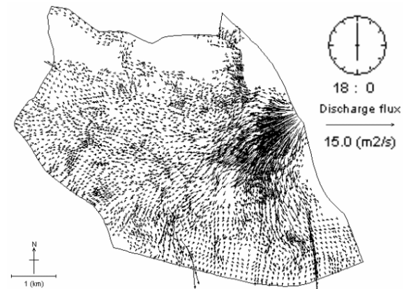
Fig.41 The discharge flux after 18 hours
