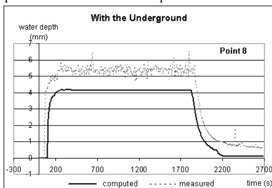
Fig.20 Comparison between the computed water depth and the measured one at point number 8
