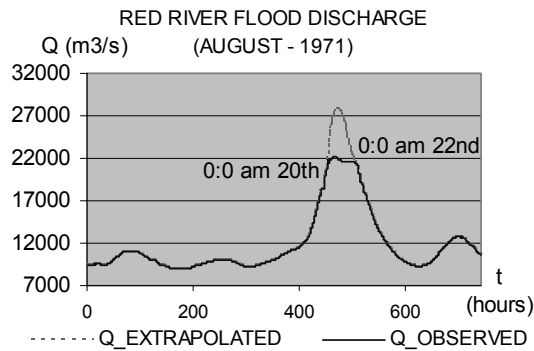
Fig.38 The observed and the extrapolated hydrographs
