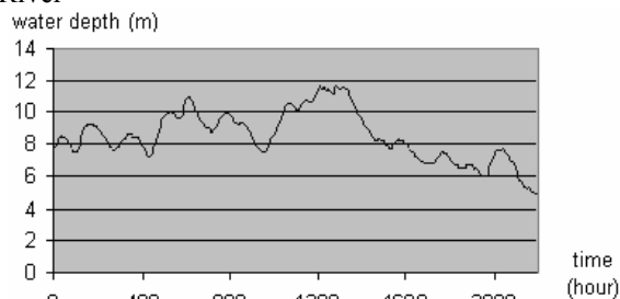
Fig.24 The observed water depth at Hanoi Station in Aug. 1996
