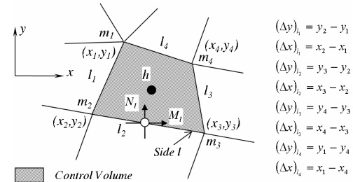
Fig.2 Control volume for continuity equation
