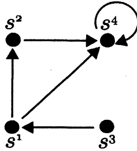
Fig. 1 The directed graph corresponding to F
