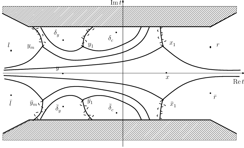
Figure 2. n = 1, m \geq 2, \text{Im } B_1(\varepsilon) > \text{Im } B_m(\varepsilon)
