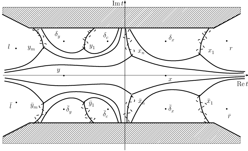
Figure 3. m \geq n \geq 2 , \text{Im } A_1(\varepsilon) > \text{Im } A_n(\varepsilon) , \text{Im } B_1(\varepsilon) > \text{Im } B_m(\varepsilon)
