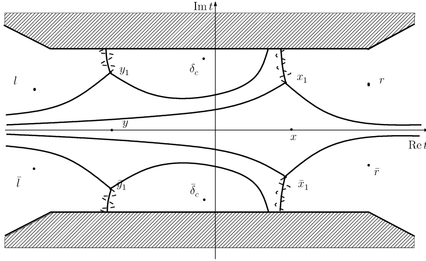
Figure 1. n = m = 1 , \text{Im } A_1(\varepsilon) < \text{Im } B_1(\varepsilon)
