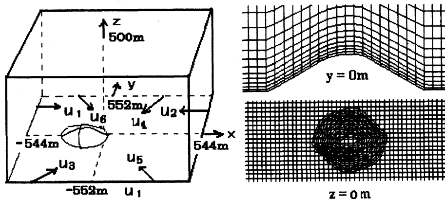
Fig.7 Computational domain (left) and the grid near the hill (right)
