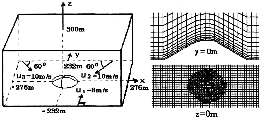
Fig.5 Computational domain (left) and the grid near the hill (right)
