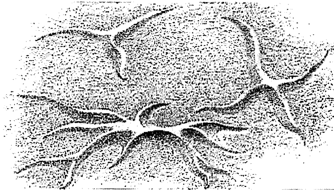
Fig.2 Star dunes 2)
