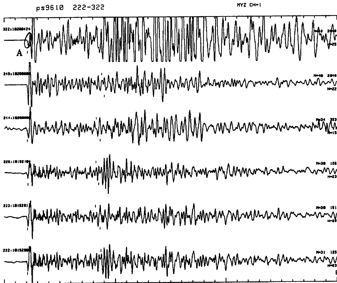
Fig. 2 The comparison of the aftershock waveforms for the Oct.1996 Hyuganada earthquake(M6.6). Each trace indicates vertical velocity obtained by short period seismograph, and is normalized by its maximum value. At the most upper trace, waveform denoted as A is different from other events waveforms.
