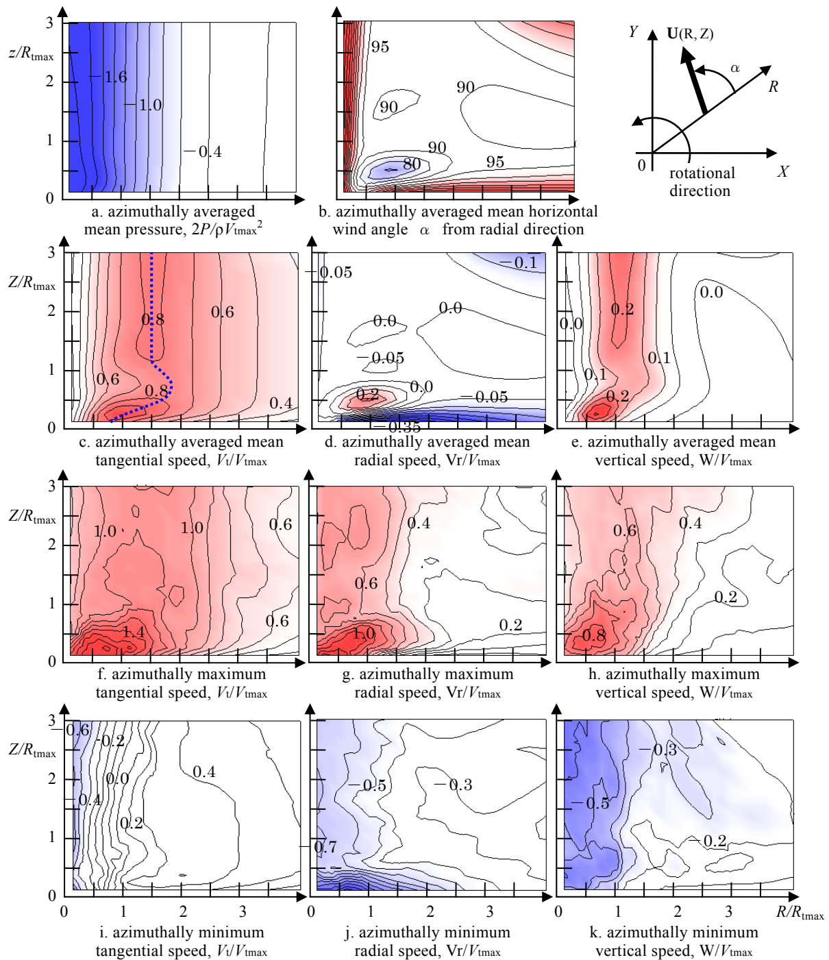
Fig. 9 Distributions of azimuthally averaged mean velocity and pressure field in a vertical plane.
