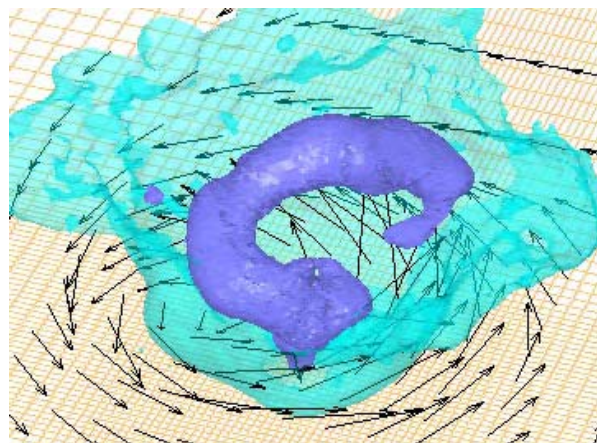
Fig. 7 Configuration and boundary conditions of calculation region with plots of instantaneous contours of low pressure regions and wind vectors near the ground ; swirling core type
