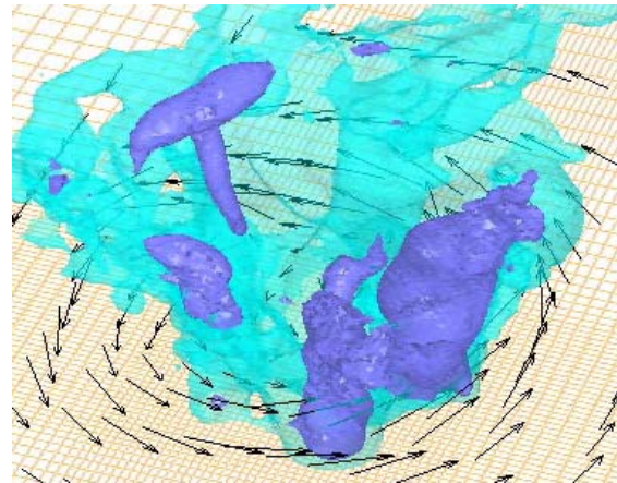
Fig. 6 Configuration and boundary conditions of calculation region with plots of instantaneous contours of low pressure regions and wind vectors near the ground ; multiple core type
