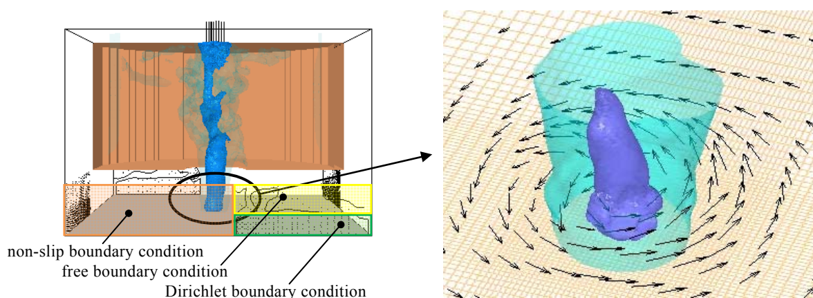
Fig. 5 Configuration and boundary conditions of calculation region with plots of instantaneous contours of low pressure regions and wind vectors near the ground ; single core type with mean down flow region in the core R_t=0.05\text{m} , R_{cnv}=0.6\text{m} , R_{ud}=0.15\text{m} , H_c=0.6\text{m} , H_d=0.2\text{m} , D=0.6\text{m} , W_o=1.0\text{m/s} , V_{tmax}=0.25\text{m/s} , Sw=0.5 , Re=760
