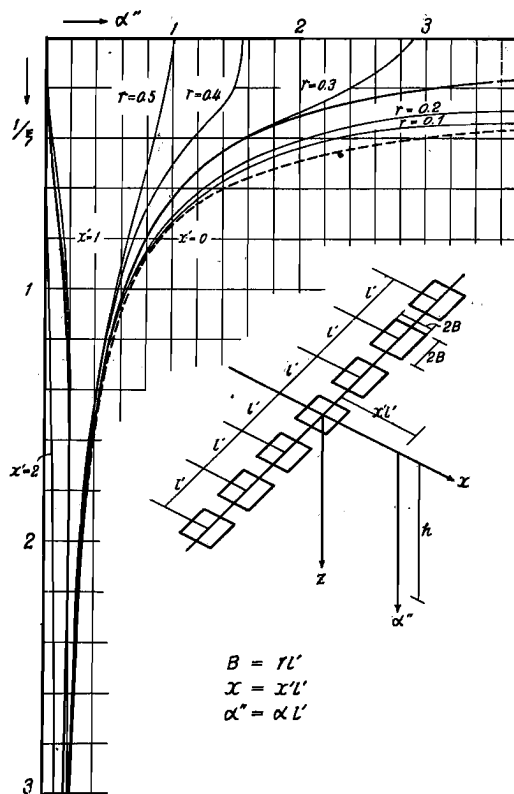
Fig. 19 The comparison among \alpha'' caused by line load (: the thick real curves), infinite series of concentrated loads (: the dashed curves) and series of square loaded plates (: the fine real curves).
