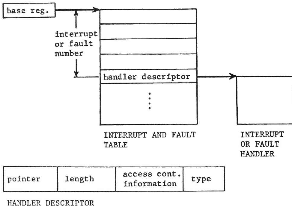
Figure 11.7 Interrupt and fault table.
