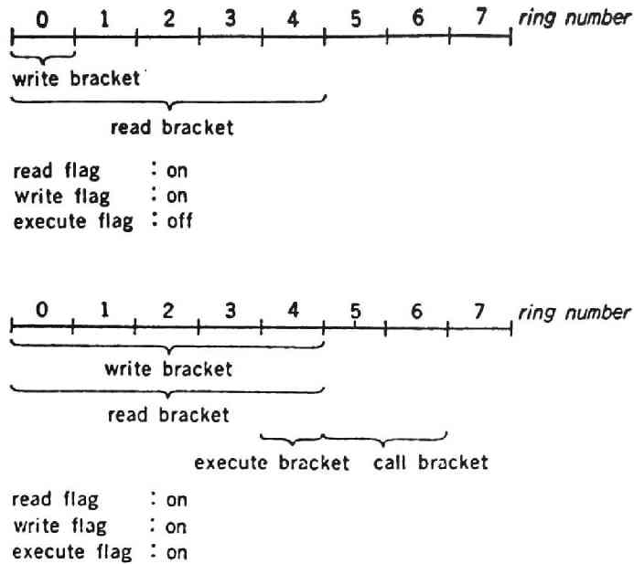
Figure 7.1 Examples of access flags and ring brackets. Bracket means the range where some access is permitted.
