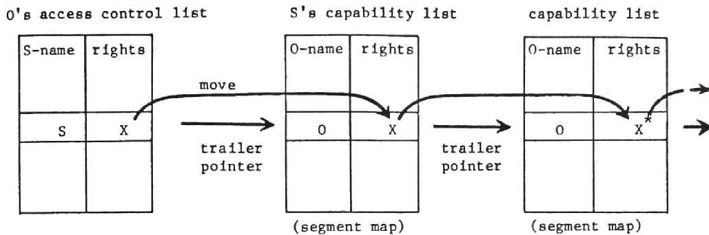
Figure 16.3 Transfer of access capability.
