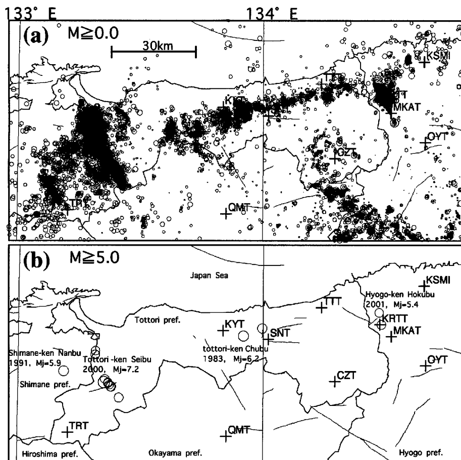
Fig. 1 (a) Seismicity around Tottori Prefecture (1997-2001, M \geq 0.0 ). (b) Earthquakes larger than M5.0 .
