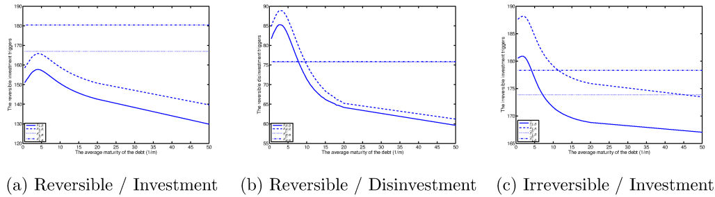
Figure 4: The level of the triggers w.r.t. debt maturity provided \sigma_H = 0.25 > \sigma_L = 0.2
