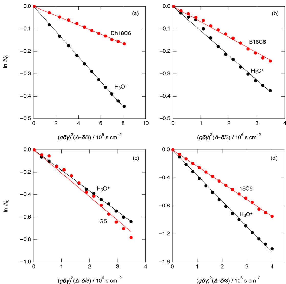
Fig. 5. Plots and best-fit lines of echo signal attenuation based on the Stejskal equation for (a) [\text{H}_3\text{O}^+ \cdot \text{Dh18C6}]\text{Tf}_2\text{N} at 70 °C, (b) [\text{H}_3\text{O}^+ \cdot \text{B18C6}]\text{Tf}_2\text{N} at 75 °C, (c) [\text{H}_3\text{O}^+ \cdot \text{G5}]\text{Tf}_2\text{N} at 25 °C, and (d) [\text{H}_3\text{O}^+ \cdot 18\text{C6}]\text{Tf}_2\text{N} at 75 °C (ref. 21): ligand (red circles) and \text{H}_3\text{O}^+ (black circles).
