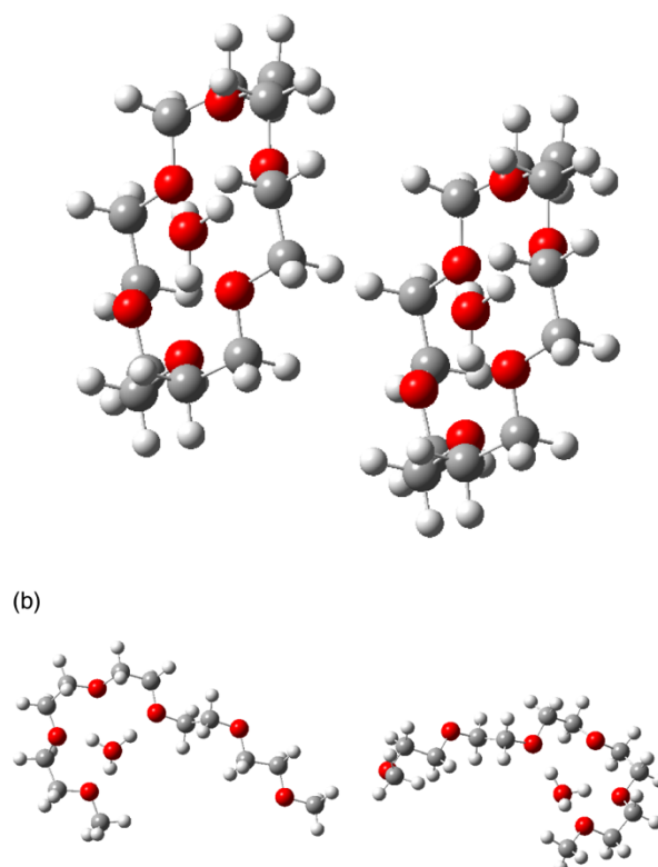
Fig. 7. Graphical representation of the equilibrium geometry of the most stable conformers of (a) two [\text{H}_3\text{O}^+\cdot\text{18C6}] cations and (b) two [\text{H}_3\text{O}^+\cdot\text{G5}] cations (B3LYP/6-311+G** level): oxygens in red, carbons in gray, and hydrogens in white.
