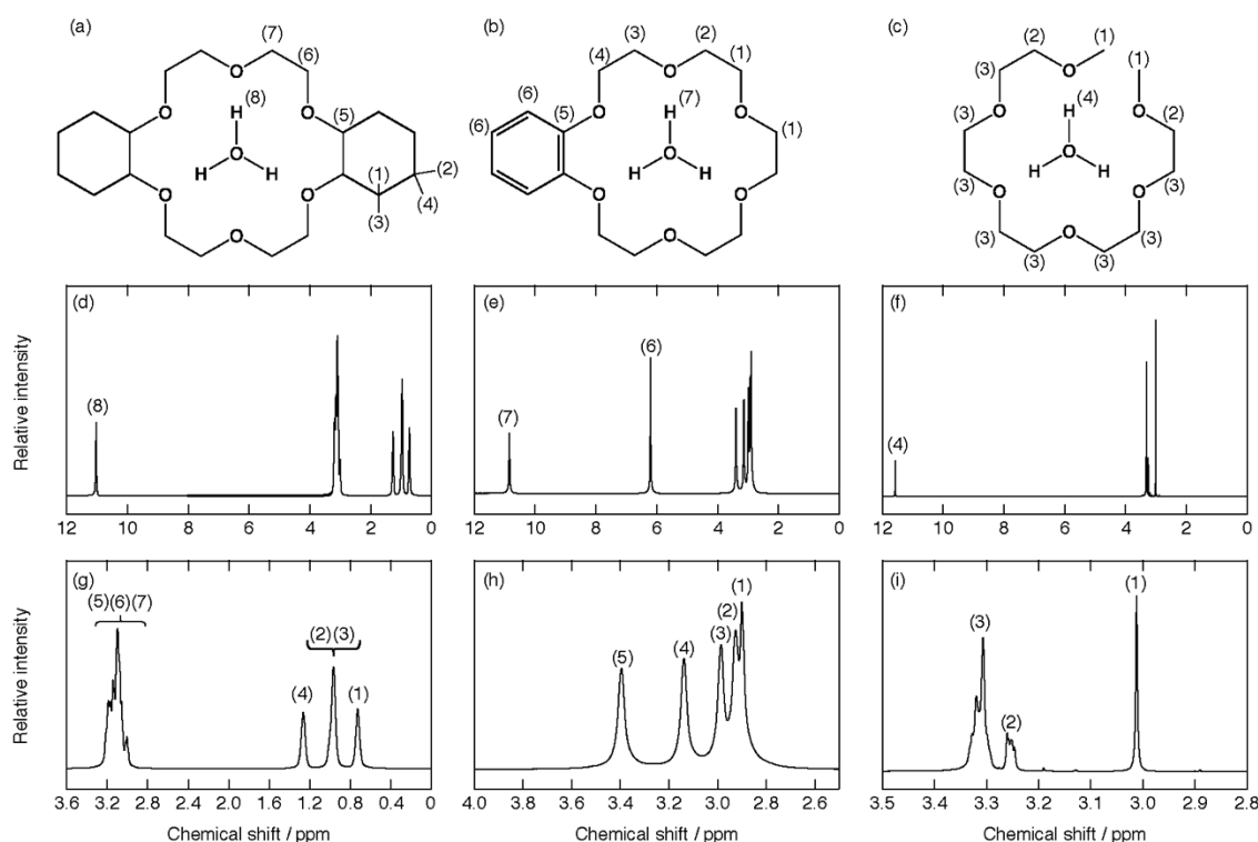
Fig. 2. (a-c) Schematic cation structure of (a) [H 3 O + ·Dh18C6], (b) [H 3 O + ·B18C6], and (c) [H 3 O + ·G5]; (d-f) ^1\text{H} NMR spectra; (g-i) enlarged plots for (d,g) [H 3 O + ·Dh18C6]Tf 2 N at 60 °C, (e,h) [H 3 O + ·B18C6]Tf 2 N at 75 °C, and (f,i) [H 3 O + ·G5]Tf 2 N at 25 °C.
