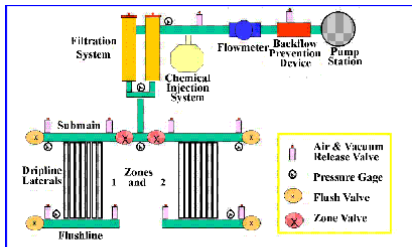
Fig. 13 Schematic of subsurface drip irrigation (SDI) system
