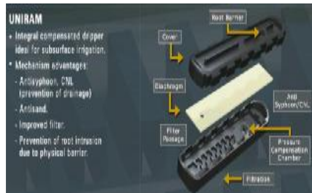
Figure 14 Structure of drippers
