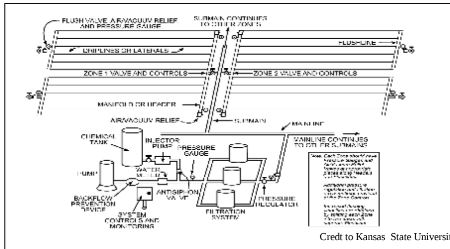
Figure 12 Schematic of a basic microirrigation system
