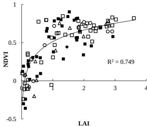
Fig. 3 Relationship between (a) back scattering coefficient (BSC) and leaf area index (LAI), (b) BSC and normalized difference vegetation index (NDVI), (c) LAI and NDVI. S: the field where BSC and DAT had a significant correlation. N: the field where BSC and DAT had a non-significant correlation. DW: the field that had more than 30 cm depth of standing water. Weed: the field covered by more than 20% weeds at the maximum.
