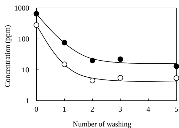
Figure 5. Influence of the number of washings of \text{NaBH}_4 -reduced Avicel PH-101 on the Na (solid circles) and B (open circles) contents after heat treatment ( \text{N}_2/240\text{ }^\circ\text{C}/30\text{ min} ). Washing condition: 0.001 N HCl (2 mL), then water ( 5\times 2\text{ mL} ).
