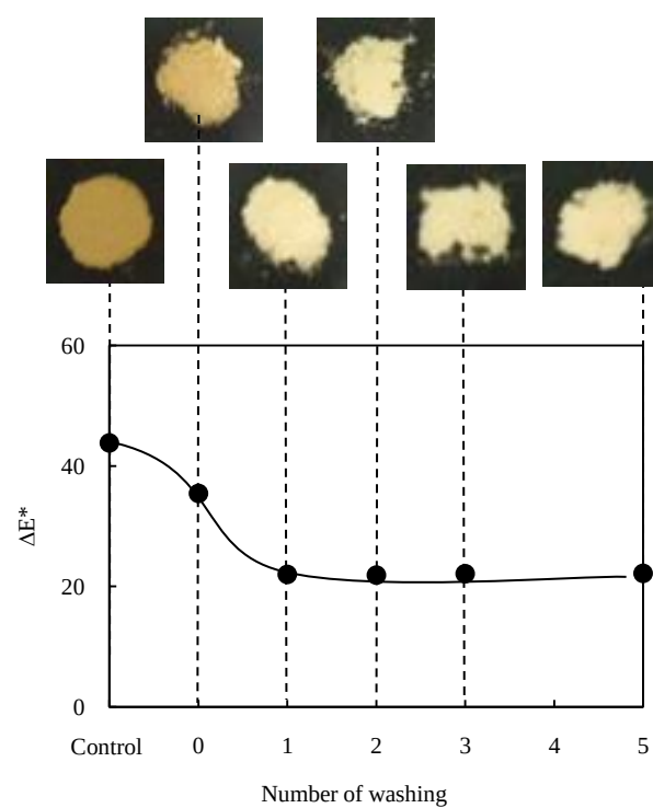
Figure 6. Influence of the number of washings of \text{NaBH}_4 -reduced Avicel PH-101 on discoloration and total color difference ( \Delta E^* ) after heat treatment ( \text{N}_2/240\text{ }^\circ\text{C}/30\text{ min} ). Washing condition: 0.001 N HCl (2 mL), then water ( 5 \times 2 mL).
