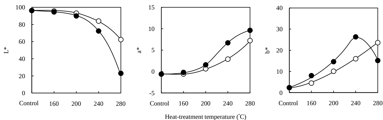
Figure 8. Changes of the CIE color parameters ( L^* , a^* , and b^* ) after heat treatment of Avicel PH-101 in the presence (open circles) or absence (closed circles) of tetraethyleneglycol dimethylether (TEGDE) under N_2 at various temperatures for 30 min. The sample preparation conditions are given in the footnote to Figure 7.
