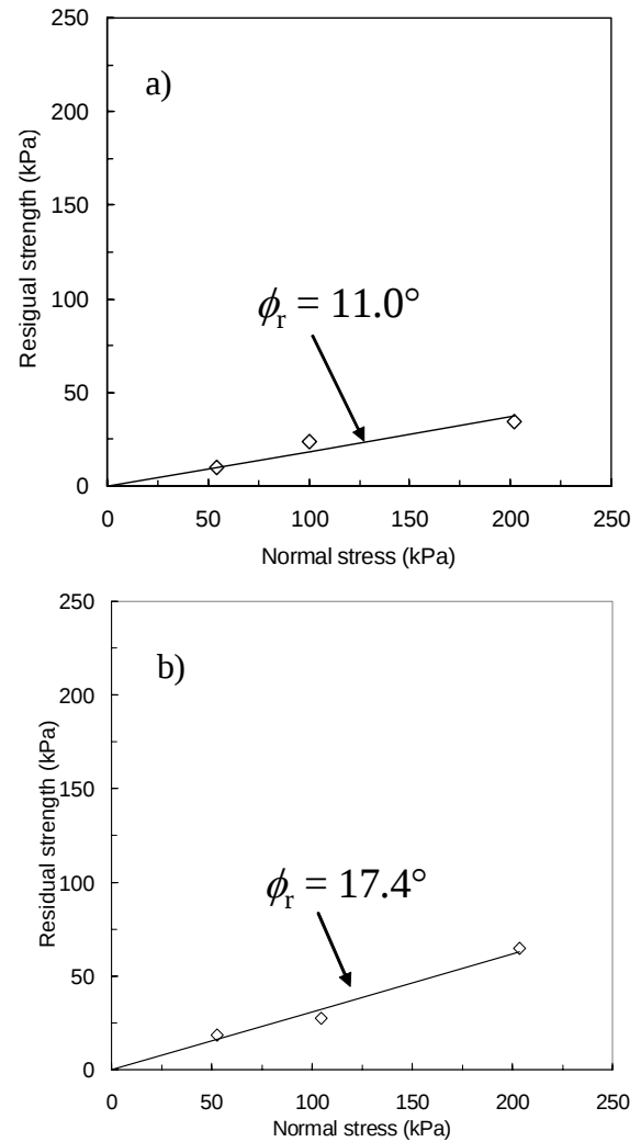
Fig. 7 Results from drained speed-controlled ring-shear tests on the soils from the “Ogotoi” landslide
