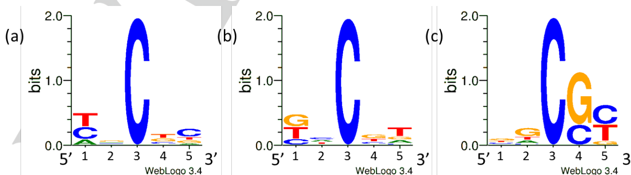
Figure 3. Reactive motif (final motif) identified from the intermediate motifs derived using Bind-n-Seq through next-generation sequencing. Randomized DNAs were incubated with (a) 6.63 \mu M, (b) 0.633 \mu M, or (c) 0.0633 \mu M Tet protein. The C in the center is mC in the original DNA sequence and hmC in the enriched sequence.
