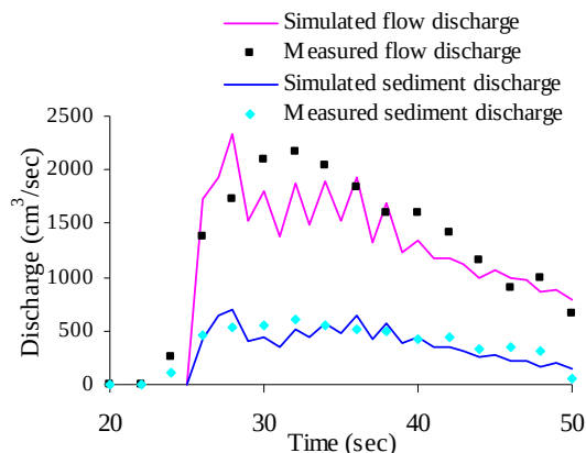
Fig. 3 Outflow hydrograph
