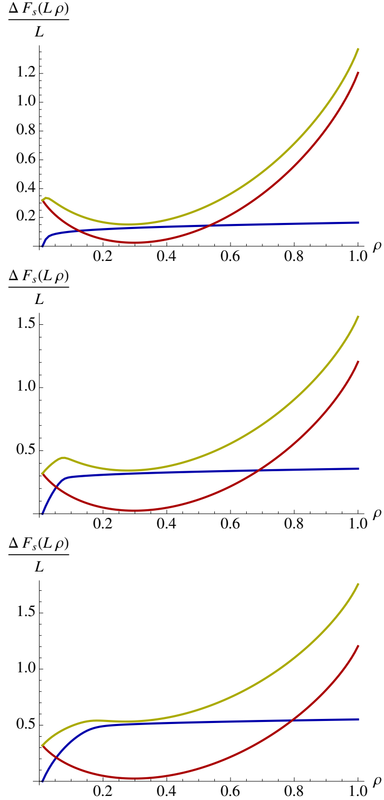
Fig. 3.4 Numerical examples of the modifying free energy \Delta F_s(\rho L)/L (blue), the modified free energy F_s(n)/L (yellow), and the original equilibrium free energy -\log P_{\text{eq}}(\rho L)/L (red) for c = 0.3, L = 100 . We set s = 0.95s_c (top), s = s_c (middle) and s = 1.05s_c (bottom).
