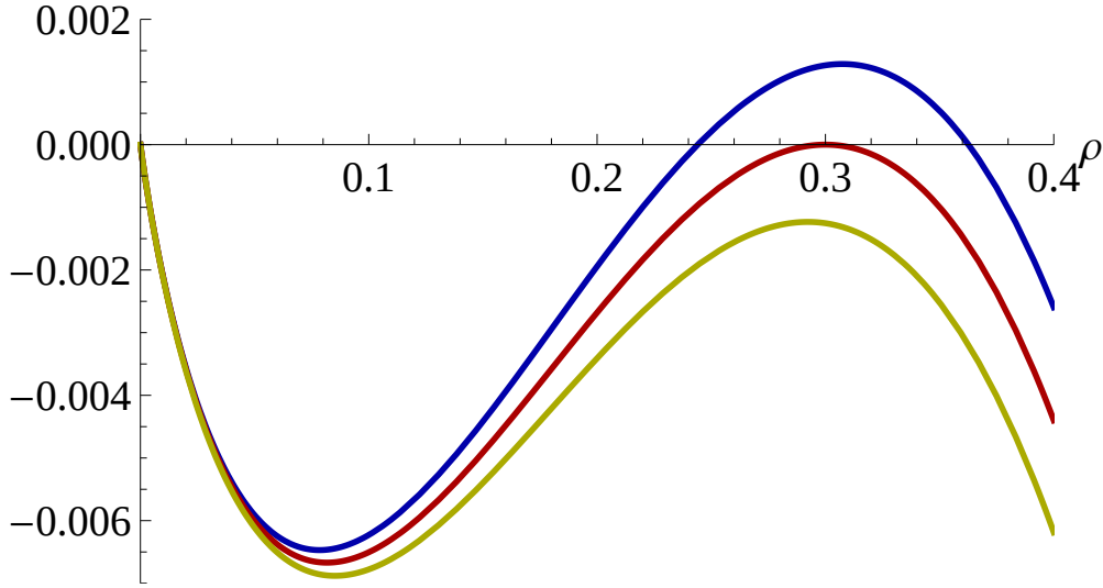
Fig. 3.1 The variational function in (3.30) as functions of \rho for several s . We set c = 0.3 . The blue, red, and yellow lines correspond to s = -0.01 , s = 0 , and s = 0.01 , respectively. One can see that \rho that maximises the function is located around c = 0.3 for s < 0 , and located around 0 for s > 0 . For s = 0 , these two phases coexist, which means that there is a first order phase transition at s = 0 .
