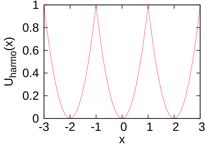
Fig. 4.1 The harmonic potential (4.8) with k = 2 and L = 1 . This is an example of the potential that satisfies the condition (4.7).
