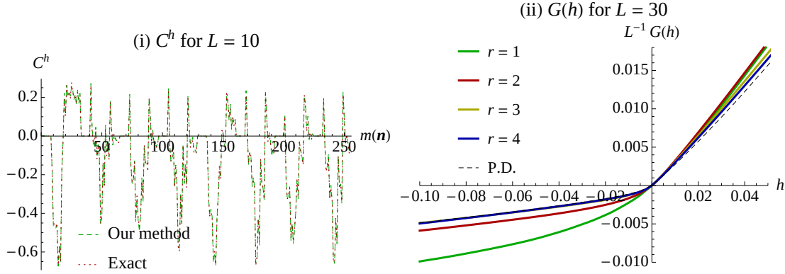
Fig. 2.10 Statistical properties of an activity for the FA model with c = 0.3 . (i) We set L = 10 , r = 4 , l = 40 and \delta h = -0.0025 , then we perform our formulation. We plot obtained C^{l\delta h}((n_{1+j})_{j=1}^r) (Our method), where the x axis represents m(\mathbf{n}) = \sum_{i=0}^{r-1} n_{L-i}2^i + \sum_{i=r}^{2r-1} n_{2r+1-i}2^i . On the same figure, we also plot \phi(C_1\mathbf{n})/\phi(\mathbf{n}) with \mathbf{n} = (0, n_2, \dots, n_{r+1}, 0, \dots, 0, n_{L-r+1}, \dots, n_L) obtained from the left eigenvector corresponding to the largest eigenvalue of L_{\mathbf{n},\mathbf{n}}^h for L = 10 with h = -0.1 (Exact). (ii) We set L = 30 and \delta h = -0.0025 , and we perform our formulation for several r . The obtained G(h)/L are plotted on the figure. At the same time, we also perform the population dynamics method [39, 40] for obtaining G(h)/L . The obtained result is plotted as a black dashed line (P. D.) in the figure.
