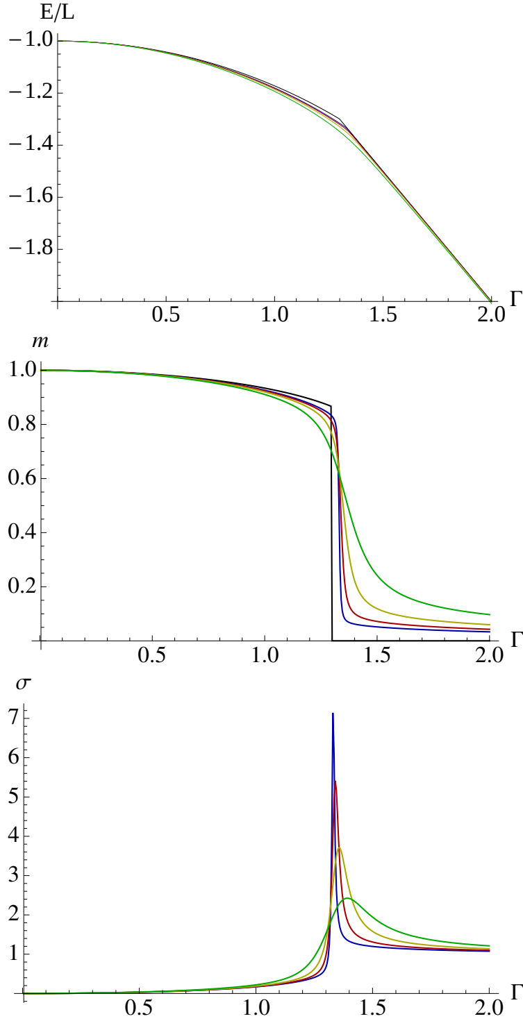
Fig. 3.13 Numerical examples of the ground state energy E/L (upper figure), the magnetisation m(\Gamma) (middle figure), and the susceptibility \sigma(\Gamma) (lower figure). Blue, red, yellow, and green lines correspond to the system size L = 50 , L = 40 , L = 30 , and L = 20 , respectively. The black lines are obtained from the variational principle (3.121), which represents the result in L \rightarrow \infty limit.
