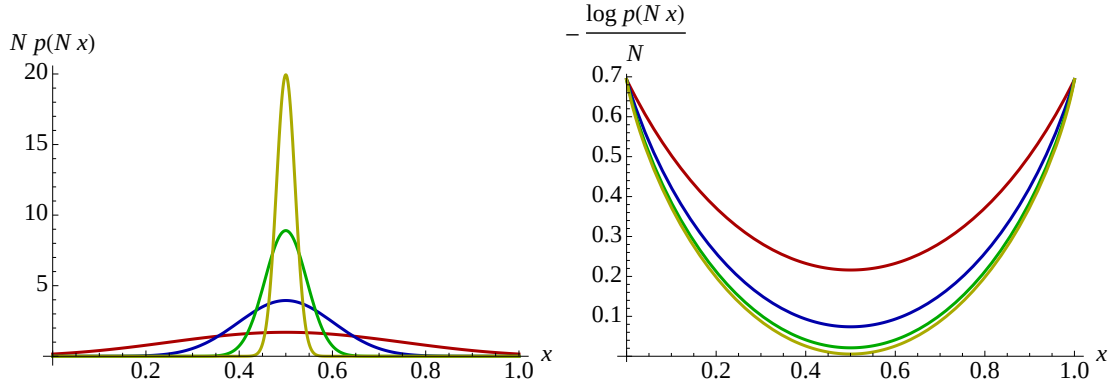
Fig. 1.1 Numerical example of p(n) given as (1.3). The left-figure is p(n) and the right-figure is the logarithm of it. The red, blue, green, and yellow lines correspond to N = 5 , N = 25 , N = 125 , and 625 , respectively.
