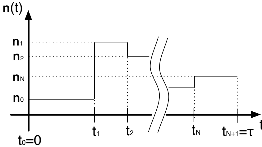
Fig. 2.1 The schematic diagram to explain the definition of the history of states, \omega .
