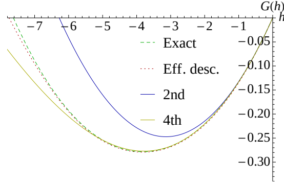
Fig. 2.7 G(h) in the open boundary ASEP obtained from our effective description. We set q = 0.5 , L = 8 , \alpha = 0.8 , \beta = 0.8 , \gamma = 0.2 , and \delta = 0.2 . Following the procedure for the effective description described in the text, we perform Monte Carlo simulations with fixed \delta h = -0.02 . The result is labeled as Eff. desc. For comparison, we also plot the largest eigenvalue of L_{\mathbf{n}, \mathbf{n}'} (Exact), the truncated cumulant expansions up to the second order: G_2(h) = hg_1 + h^2g_2 (2nd) and the fourth order: G_4(h) = hg_1 + h^2g_2 + h^3g_3 + h^4g_4 (4th), where the coefficients g_i are defined as (1/i!)\partial^i G(h)/\partial h^i|_{h=0} . These coefficients are calculated from the exact formula in Refs. [23, 24].
