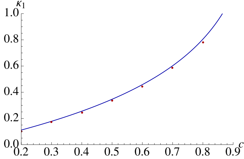
Fig. 3.11 Numerical check of the formula giving \kappa (3.85). We estimated (1/L) \log \kappa for c = 0.2, 0.3, \dots, 0.8 from the fitting lines in Fig. 3.9 and plot them with red dots. On the same figure, we draw the analytical result -\frac{1}{2} \log(1-c) with blue line. The agreement is relatively good although red dots are obtained from finite size L .
