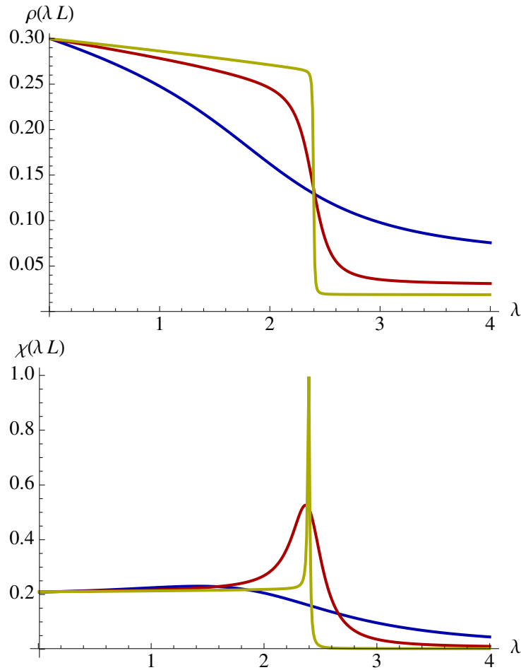
Fig. 3.3 The modified magnetisation \rho(s) (upper) and the modified susceptibility \chi(s) (lower) given in (3.38) and (3.39) as functions of \lambda = s/L . We numerically solve the largest eigenvalue problem (3.19), construct the distribution function P^s(n) from (3.34), and calculate \rho(s) and \chi(s) . We set c = 0.3 , and L = 20 (blue), L = 40 (red), L = 60 (yellow). We note that the position of the peak of \chi(s) is equal to s_c(L) defined in (3.31), so that it close to \lambda_c = 1/(2c(1-c)) due to (3.32). Indeed, from the figure, we estimate it as \lambda = 2.398\dots for L = 60 , to which the corresponding \lambda_c is 2.381\dots
