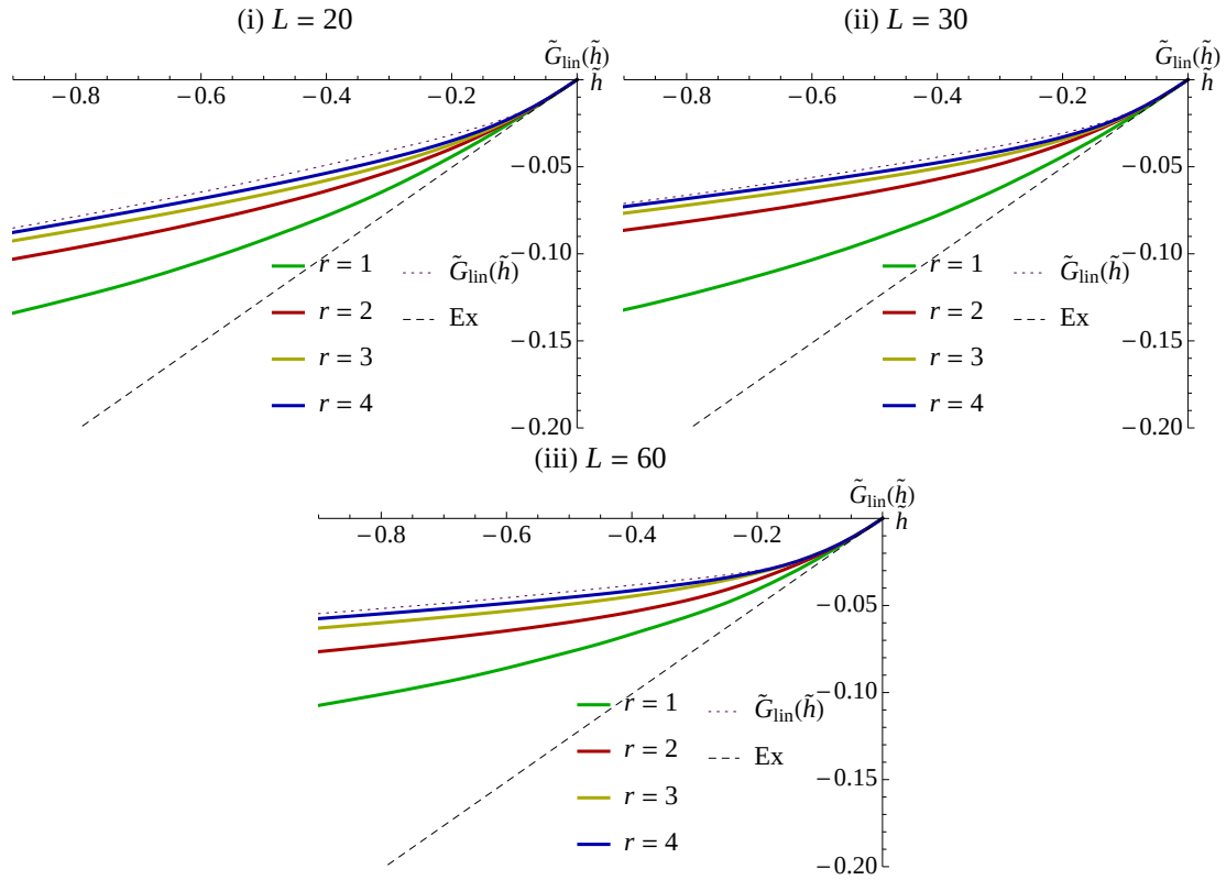
Fig. 2.13 \tilde{G}(\tilde{h}, r) and \tilde{G}_{\text{lin}}(\tilde{h}) for r = 1, 2, 3, 4 with L = 20 (i), 30 (ii), and 60 (iii), where we set c = 0.3 .
