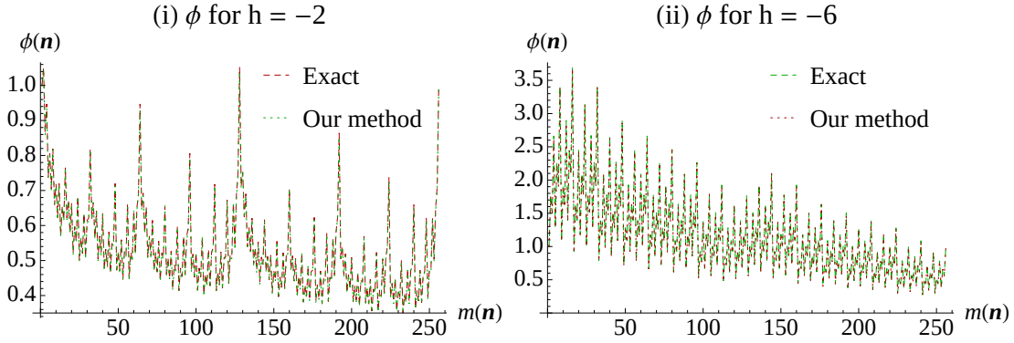
Fig. 2.5 Numerical check of our formulation for the open boundary ASEP. We set q = 0.5 , L = 8 , \alpha = 0.8 , \beta = 0.8 , \gamma = 0.2 , and \delta = 0.2 . We perform our computational method on Monte Carlo simulations with setting l = 100 and 300 with \delta h = -0.02 . The obtained \prod_{k=0}^{l-1} \left\langle e^{\tau \delta h A(\omega)} \right\rangle_{\mathbf{n}}^{k \delta h} are plotted on (i) (for l = 100 ) and (ii) (for l = 300 ) labeled as our method. In the figure, the x axis represents m(\mathbf{n}) = \sum_{i=0}^{L-1} n_{L-i} 2^i , which is the decimal value of the binary number \mathbf{n} . On the same figures, we also plot \phi(\mathbf{n}) that is the left eigenvector corresponding to the largest eigenvalue of L_{\mathbf{n}', \mathbf{n}}^h defined in (2.25) for h = -2 and h = -6 (Exact). In these two figures, we can see the coincidence very well between \prod_{k=0}^{l-1} \left\langle e^{\tau \delta h A(\omega)} \right\rangle_{\mathbf{n}}^{k \delta h} and \phi(\mathbf{n}) .
