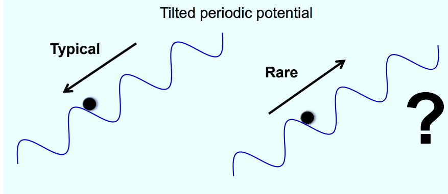
Fig. 1.3 Schematic picture of a Brownian particle on a tilted periodic potential. Most of the time, the particle goes down the potential as shown in the left figure, however, the probability of the particle climbing up the potential is not 0.
