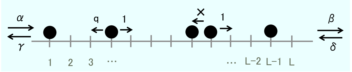
Fig. 2.4 Schematic picture representing the definition of ASEP
