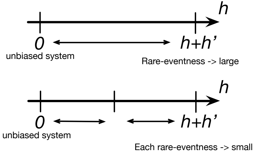
Fig. 2.2 The schematic diagram for renormalisability of rare-eventness.
