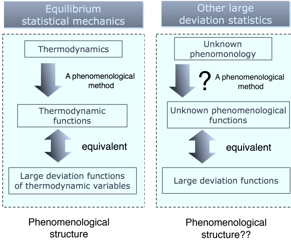
Fig. 1.2 Schematic picture representing phenomenological structure for large deviation principle.
