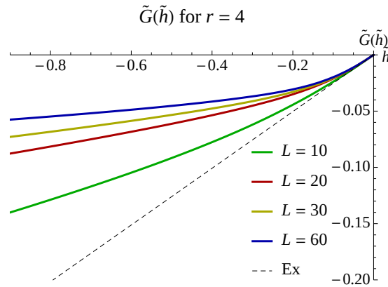
Fig. 2.14 \tilde{G}(\tilde{h}) for various values of L with r = 4 fixed. We also plot the straight line (Ex) of slope 4c^2(1-c) that corresponds to the expected value of the activity in the unbiased system ( h = 0 ).
