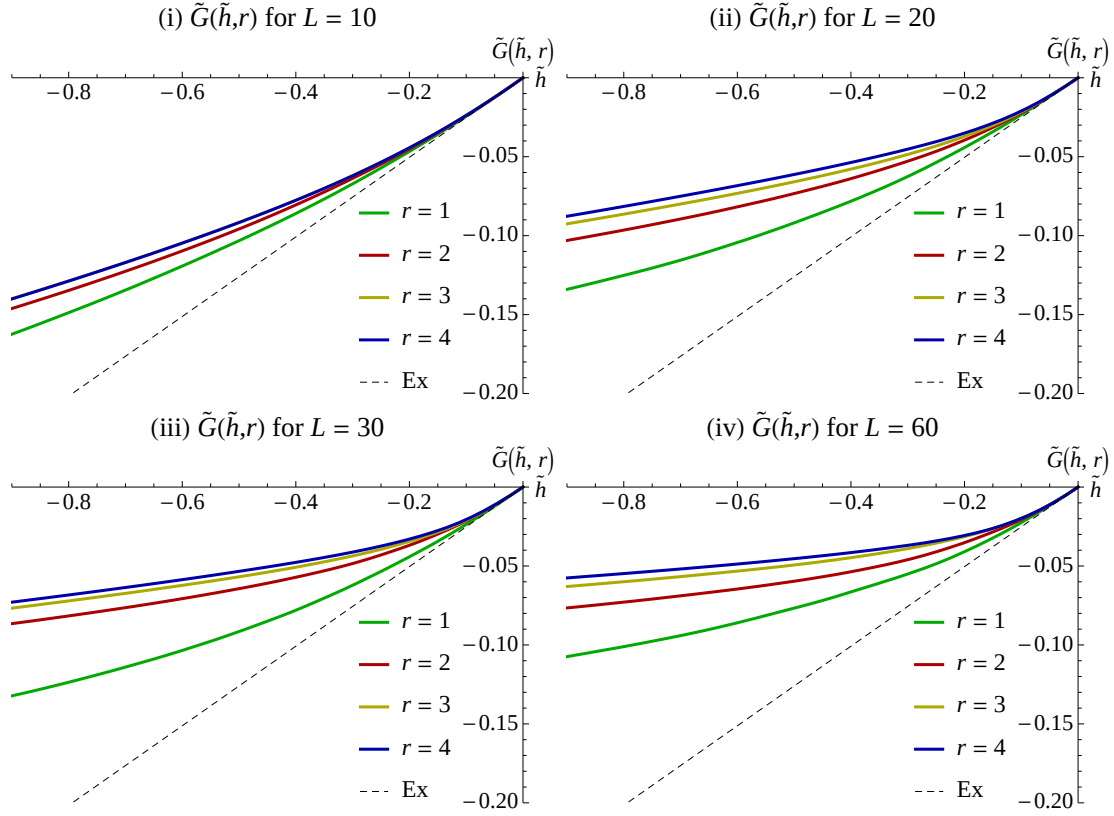
Fig. 2.11 \tilde{G}(\tilde{h}, r) for r = 1, 2, 3, 4 with L = 10 (i), 20 (ii), 30 (iii), and 60 (iv), where we set c = 0.3 . We also plot the straight line of slope 4c^2(1 - c) (Ex) in each figure, which corresponds to \tilde{G}(\tilde{h}, 0) .
