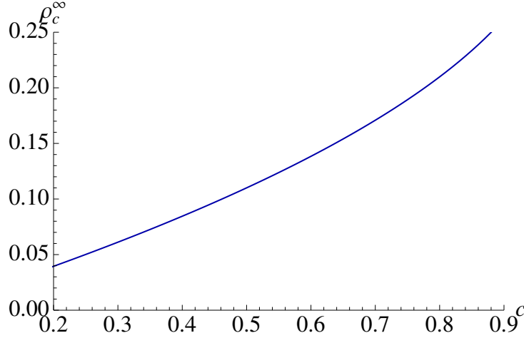
Fig. 3.5 Connecting point \rho_c^\infty given as (3.52). We numerically solve (3.52) and plot it as a function of c .
