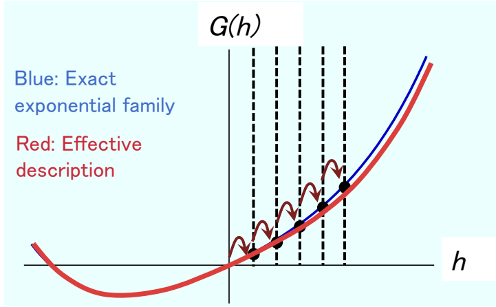
Fig. 2.3 Schematic picture explaining the effective description of exponential family.
