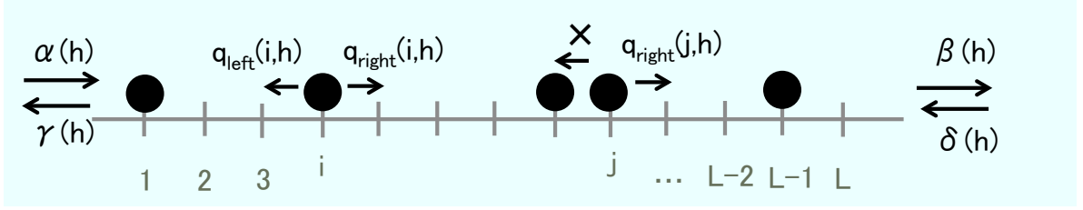
Fig. 2.6 An example of an effective description for ASEP. In this figure, each transition rate is given as follows: q_{\text{left}}(i, h) = qe^{-h/(L-1)}\psi_{h,i-1}/\psi_{h,i} , q_{\text{right}}(i, h) = qe^{h/(L-1)}\psi_{h,i+1}/\psi_{h,i} , \alpha(h) = \alpha\psi_{h,1}/\psi_{h,0} , \gamma(h) = \gamma\psi_{h,0}/\psi_{h,1} , \beta(h) = \beta\psi_{h,0}/\psi_{h,L} and \delta(h) = \delta\psi_{h,L}/\psi_{h,0} .
