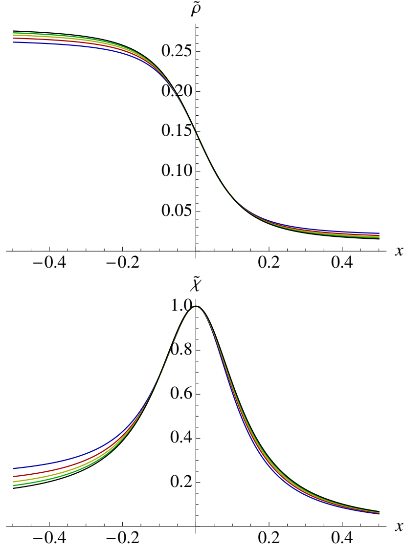
Fig. 3.10 Numerical examples of the rescaled magnetisation \tilde{\rho}(x) (upper) and the rescaled susceptibility \tilde{\chi}(x) (bottom). We set c = 0.3 , and L = 60 (blue), L = 70 (red), L = 80 (green), L = 90 (yellow), and L = 100 (black).
