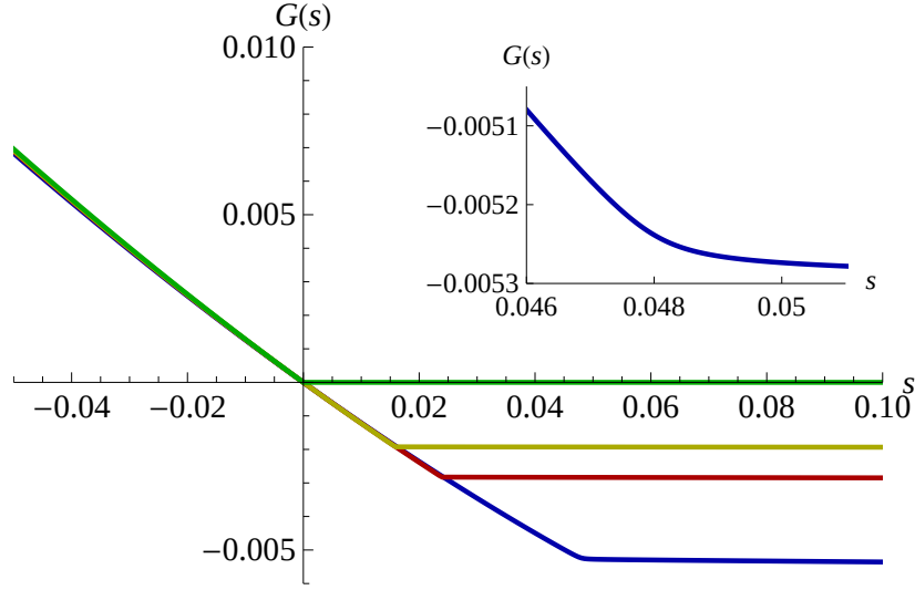
Fig. 3.2 Dynamical free energy G(s) for c = 0.3 obtained from the variational formula (3.30) (green), and numerical diagonalisation of (3.20) for L = 50 (blue), L = 100 (red), L = 150 (yellow). The inset is a magnified picture of the blue line ( L = 50 ) around the cusp, which shows the rounding of it due to the finite-size effect. We estimate the numerical examples of s_c(L) defined by (3.31). For L = 50 , L = 100 , and L = 150 , these are 0.0479..., 0.02390..., and 0.01591..., respectively. These values are close to 1/(2Lc(1 - c)) due to the formula (3.32). Indeed, 1/(2Lc(1 - c)) takes 0.04762..., 0.02381... and 0.01587... for L = 50, 100 , and 150, respectively.
