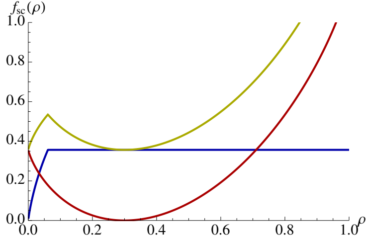
Fig. 3.6 Analytical expression of the modifying free energy for s = s_c given as (3.49) and (3.50). We plot it with blue line. We also plot the corresponding modified free energy given as f_e(\rho) + \Delta f_{s_c}(\rho) with yellow line, and the unbiased equilibrium free energy f_e(\rho) with red line.
