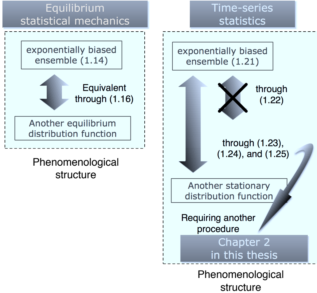
Fig. 1.4 Schematic picture explaining what we will develop in Chapter 2.
