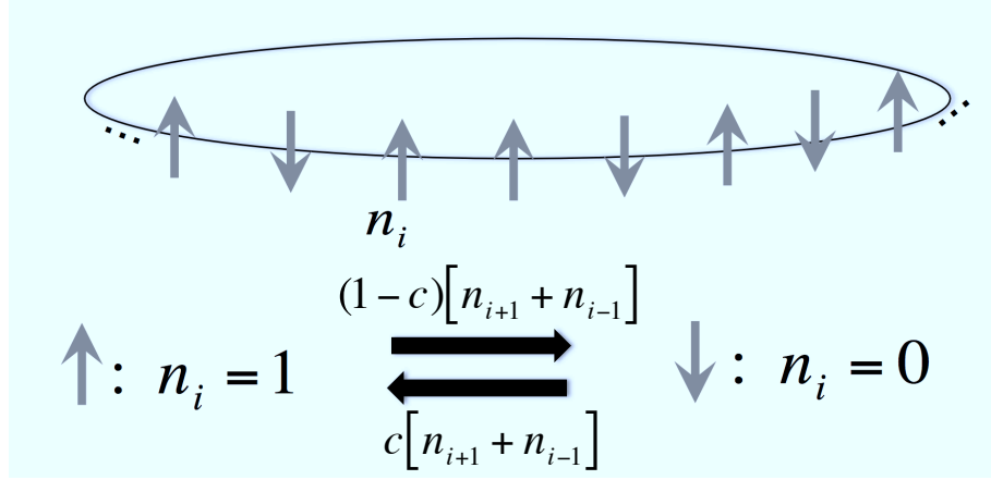
Fig. 2.8 Schematic picture explaining FA model
