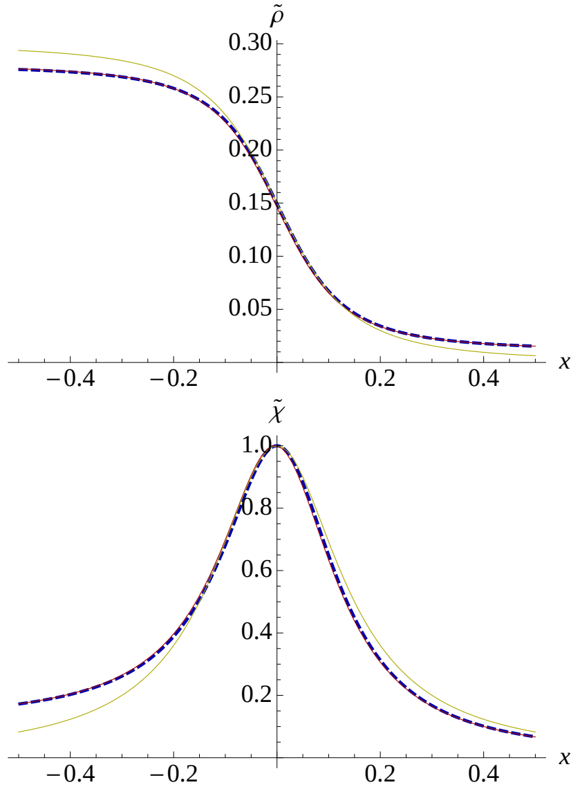
Fig. 3.12 Numerical check of the analytical expressions of the rescaled magnetisation \tilde{\rho}(x) given in (3.87) (upper figure) and the susceptibility \tilde{\chi}(x) given in (3.88) (lower figure). We set c = 0.3 and L = 100 . The solid red lines are the analytical results, and the dashed blue lines are the corresponding numerical results obtained from the diagonalisation of the matrix L_{n,n'}^s . On the same figure, for a comparison, we also plot the infinite-size scaling functions (3.89) and (3.90) with yellow solid lines. The deviation of yellow lines from the others shows the importance of the finite size corrections in (3.87) and (3.88).
