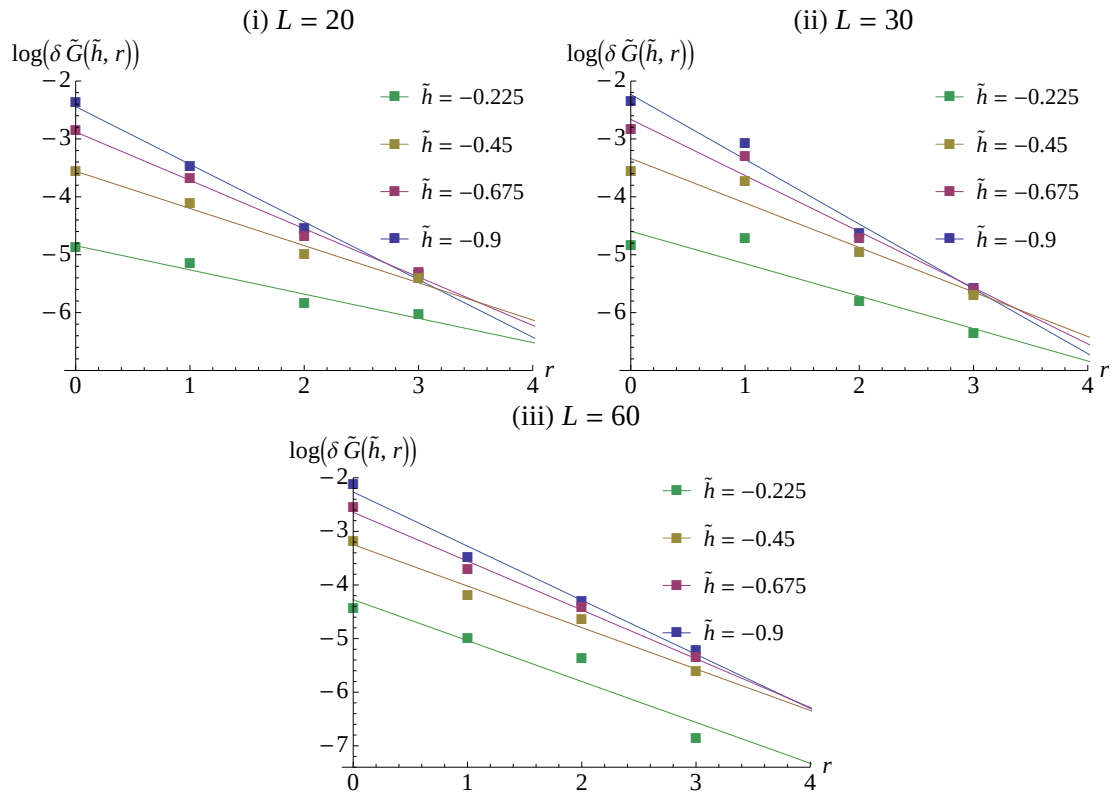
Fig. 2.12 The logarithm of the difference function \delta \tilde{G}(\tilde{h}, r) for r = 0, 1, 2 , and 3 with L = 20 (i), 30 (ii), and 60 (iii). We set c = 0.3 . We also plot straight lines obtained from a least squares fit of those data points.
