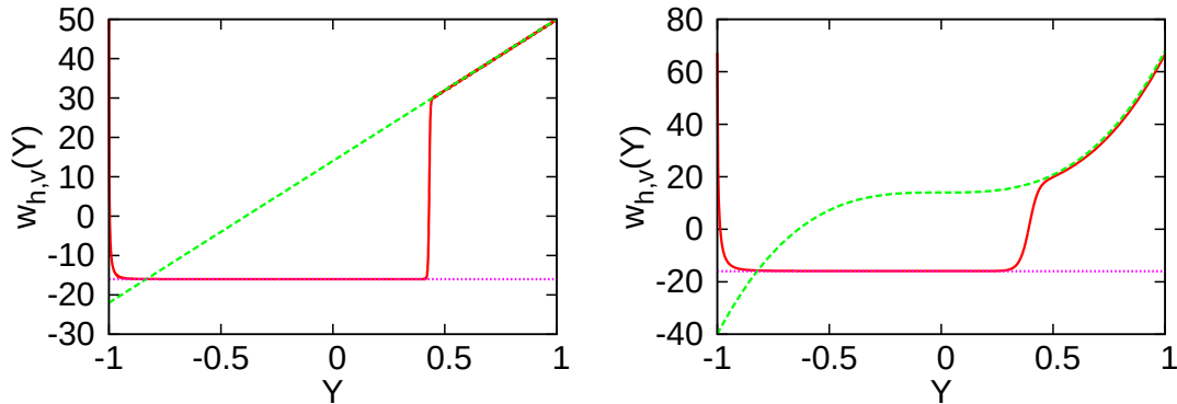
Fig. 4.2 Numerical and analytical results of \tilde{w}_{h,v}(Y) for the harmonic and quartic potentials U_{\text{harmonic}}(y) = (k/2)y^2 (left) and U_{\text{quartic}}(y) = (k_4/4)y^4 (right). Quantities are converted to dimensionless forms with setting \gamma = T = v = 1 . We set k = 1 , k_4 = 1 and h = -8 , and also, we set L = 18 for U_{\text{harmonic}}(y) and L = 3 for U_{\text{quartic}}(y) . The green dashed lines and purple dotted lines corresponds to the analytical results (4.83). These lines are 14 + 36Y and -16 for U_{\text{harmonic}}(y) , and 14 + 54Y^3 and -16 for U_{\text{quartic}}(y) . The red solid lines are numerical results.
