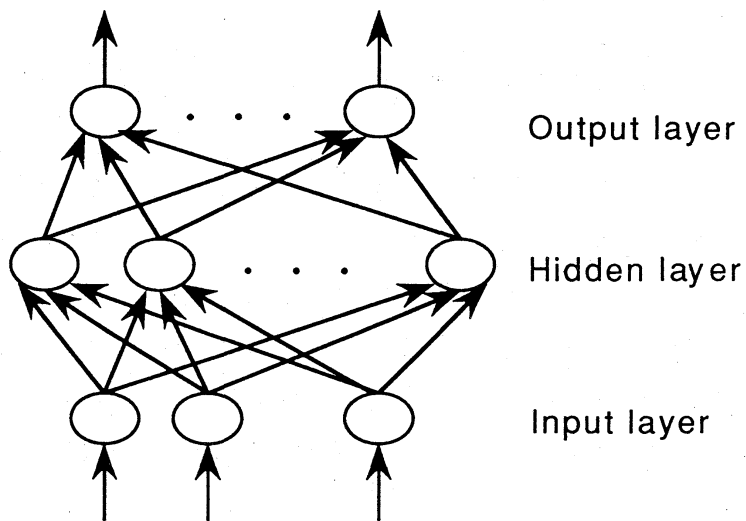
Figure 2. Three-layer feedforward network
