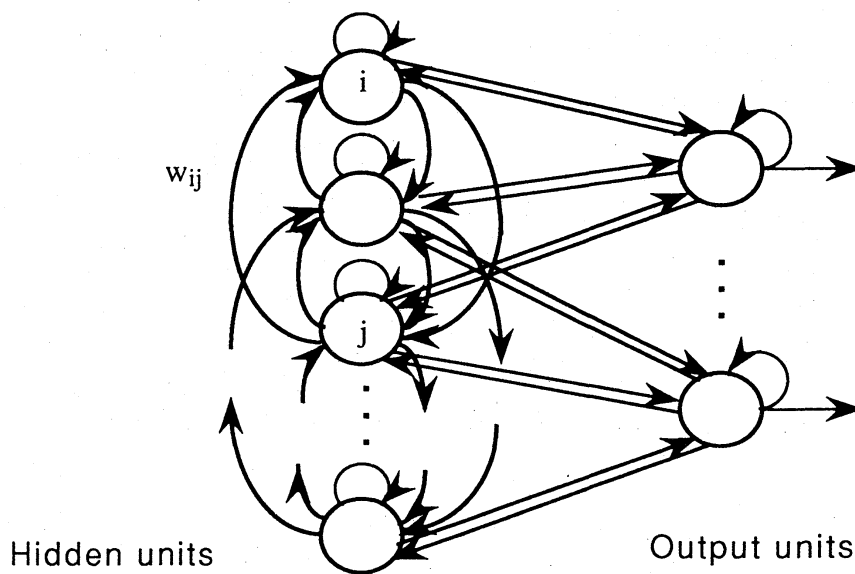
Figure 3. Recurrent neural network
