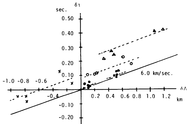
Fig. 10. Difference of the epicentral distances versus the reduced arrival times referred to the seismic station A at Kawanishi.
