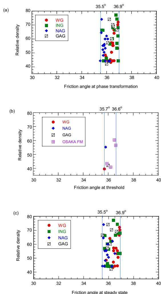
Fig. 3. Relationship between friction angle at phase transformation, threshold state, and steady state and relative density
