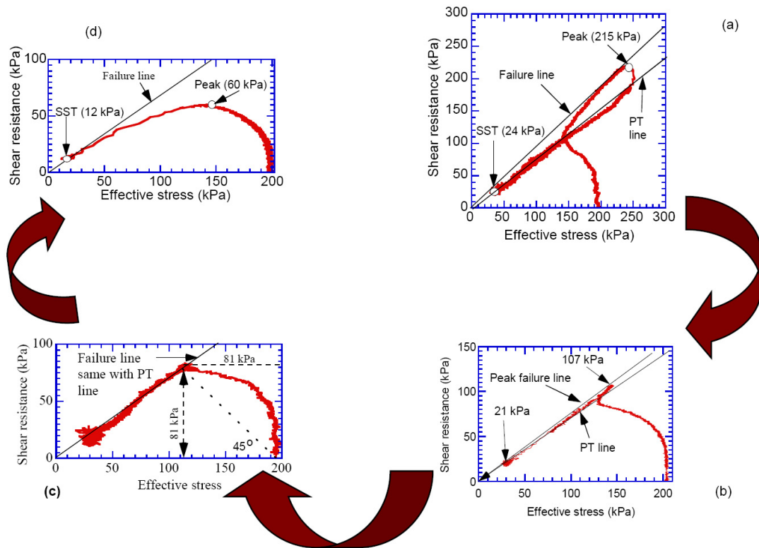
Fig. 2. The proposed soil transition route from dense to loose state: (a, b, d) well-known stress paths (c) less-known stress path
