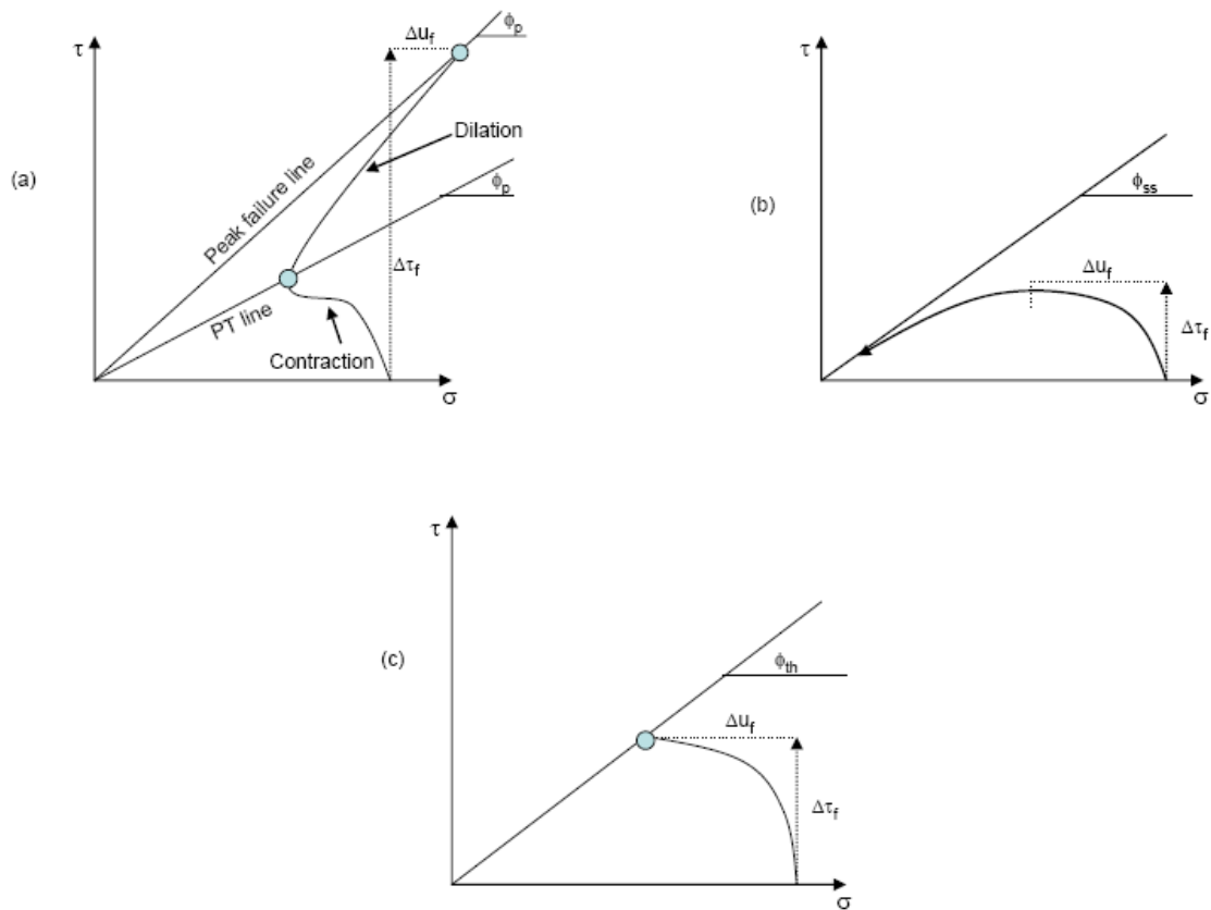
Fig. 6 The theory of threshold pore pressure
