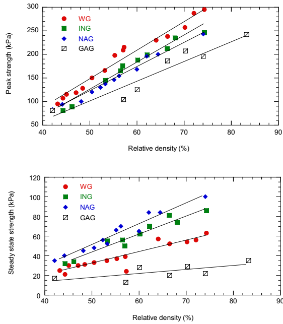
Fig. 4 The relationship between relative density and shear strength (a) peak strength (b) steady
