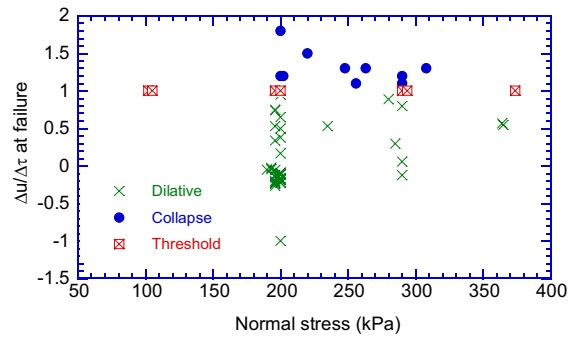
Fig. 1 The boundary between contraction and dilation
