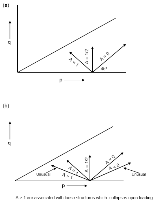
Fig . 5 Special values of A (Skempton 1954)
