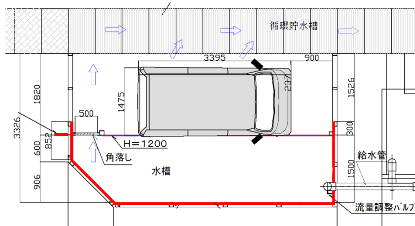
Fig. 1 Experimental set-up
