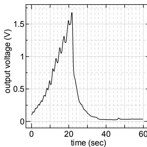
Fig. 2 Measurement result of pulling force
