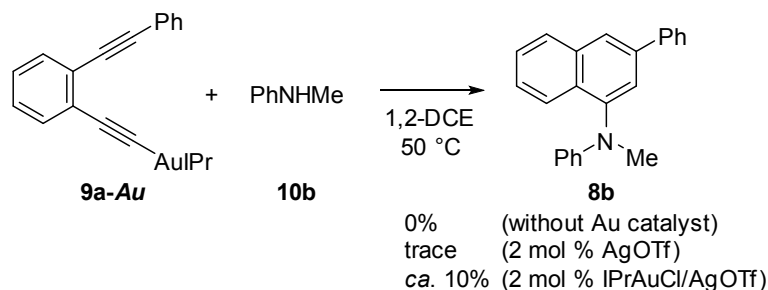
Scheme 9. Conversion of Gold Acetylide Complex 9a-Au
