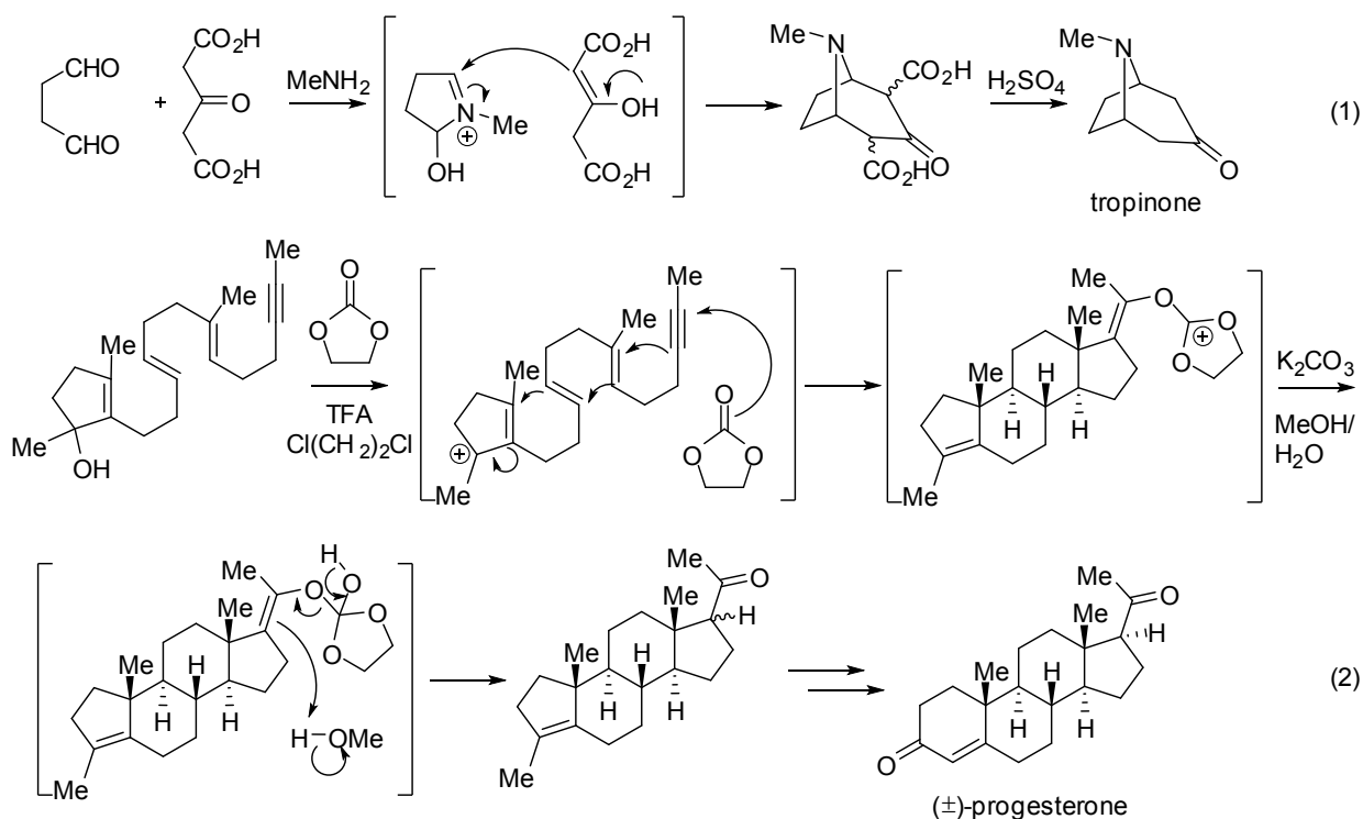
Scheme 1. Total Synthesis of Tropinone (eq 1) and (±)-Progesterone (eq 2) Based on Cascade Cyclizations
