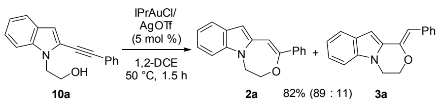
Scheme 5. Reaction of the Possible Intermediate 10a
