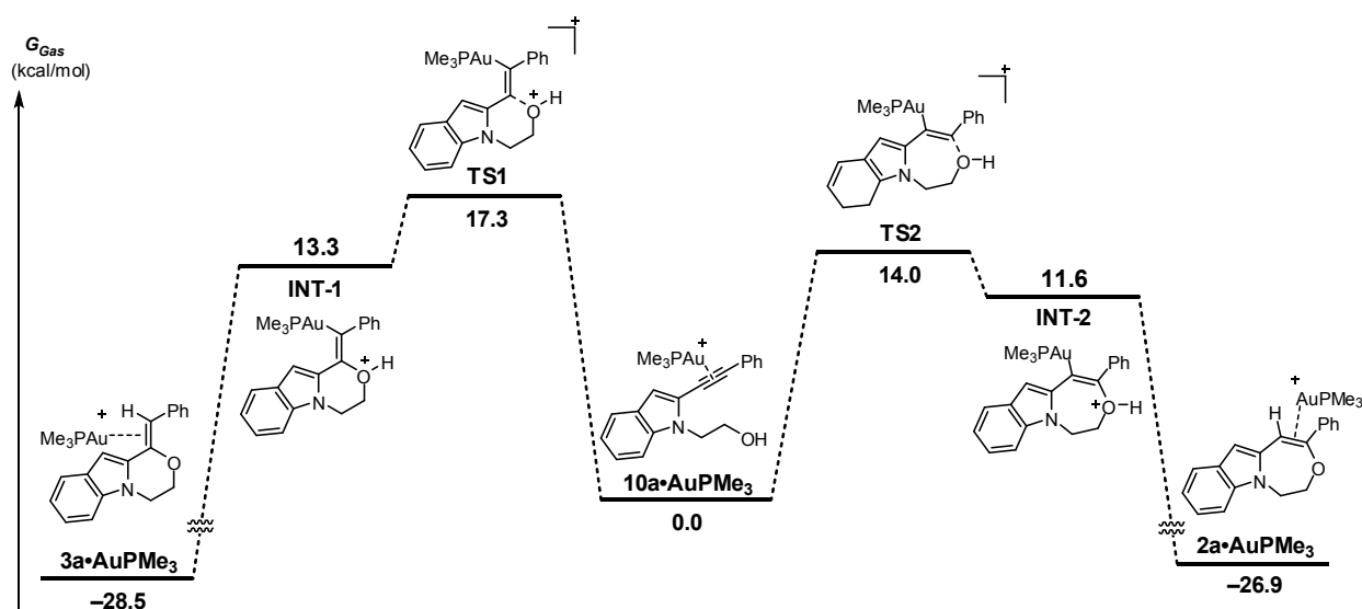
Figure 2. DFT calculations on cyclization of 10a [M06-2X/6-31G(d,p)&SDD(Au)].
