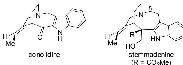
Figure 1. Stemmadenine-Based Alkaloids
