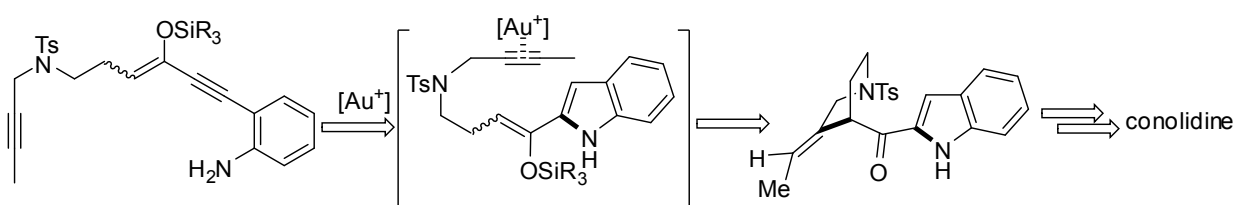
Scheme 10. The Author's Strategy (3-2): The Second Strategy for the Total Synthesis of Conolidine by Cascade Cyclization of Conjugated Enyne
