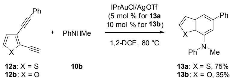
Scheme 10. Reaction of Heteroaromatic Compounds
