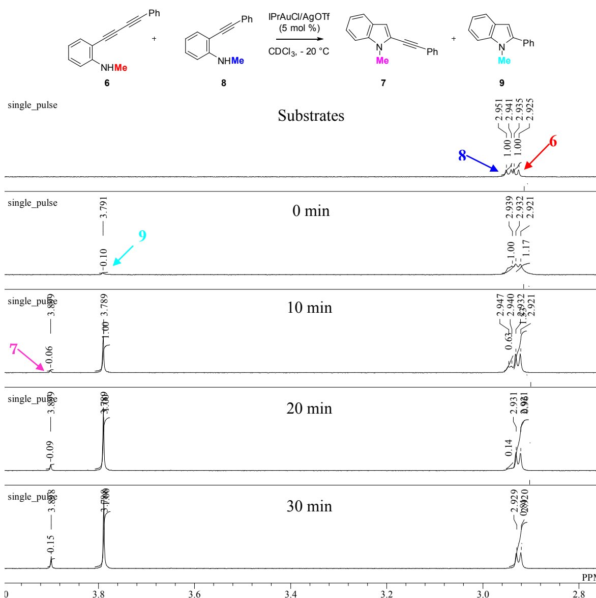
Figure 3. ^1\text{H} NMR Experiment Chart of Comparison of the Reactivities toward Indole Formation between Diynylaniline 6 and (Phenylethynyl)aniline 8
