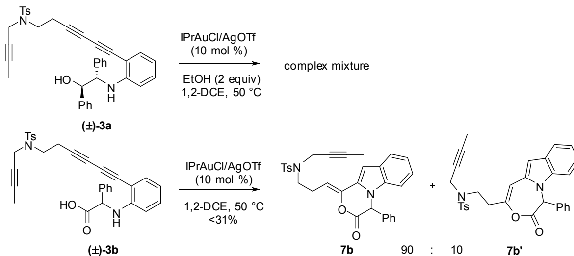
Scheme 4. Gold(I)-Catalyzed Cascade Reaction of (±)-3a and (±)-3b
