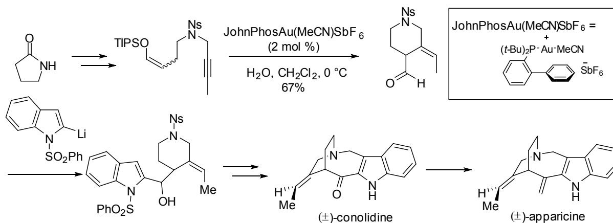
Scheme 11. Total Synthesis of (±)-Conolidine and (±)-Apparicine Reported by Takayama et al.
