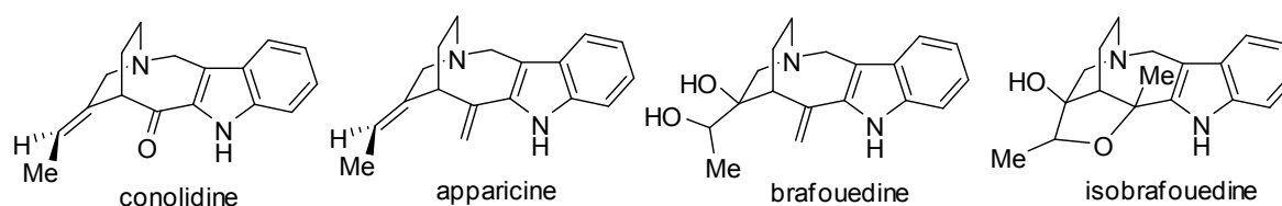
Figure 1. Structures of C5-Nor Stemmadenine-Type Indole Alkaloids
