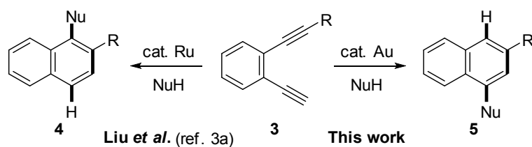
Scheme 3. Liu's Work and This Work
