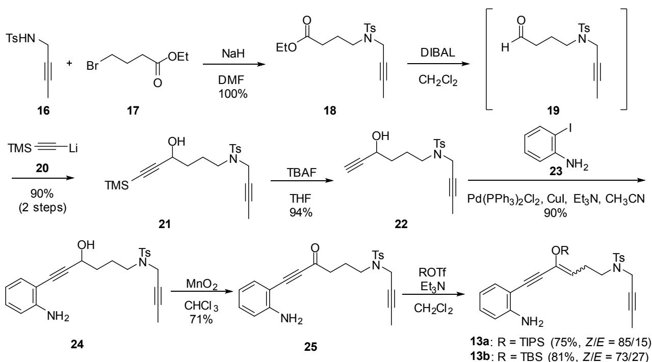
Scheme 6. Preparation of the Conjugated Enynes 13
