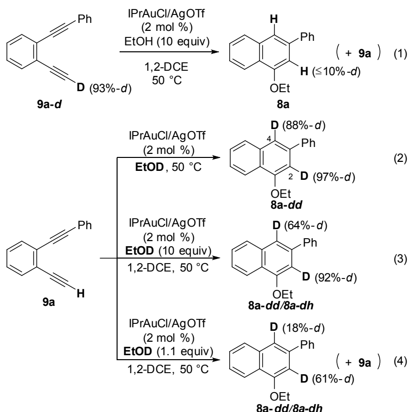
Scheme 7. Isotopic Labeling Experiments
