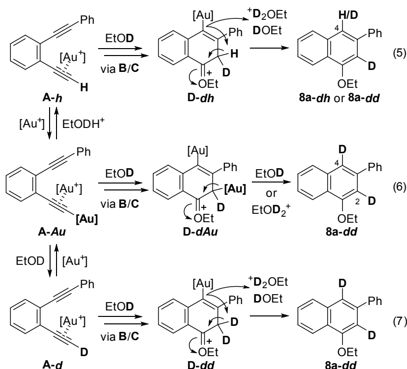
Scheme 8. Proposed Mechanism by the Experimental Results
