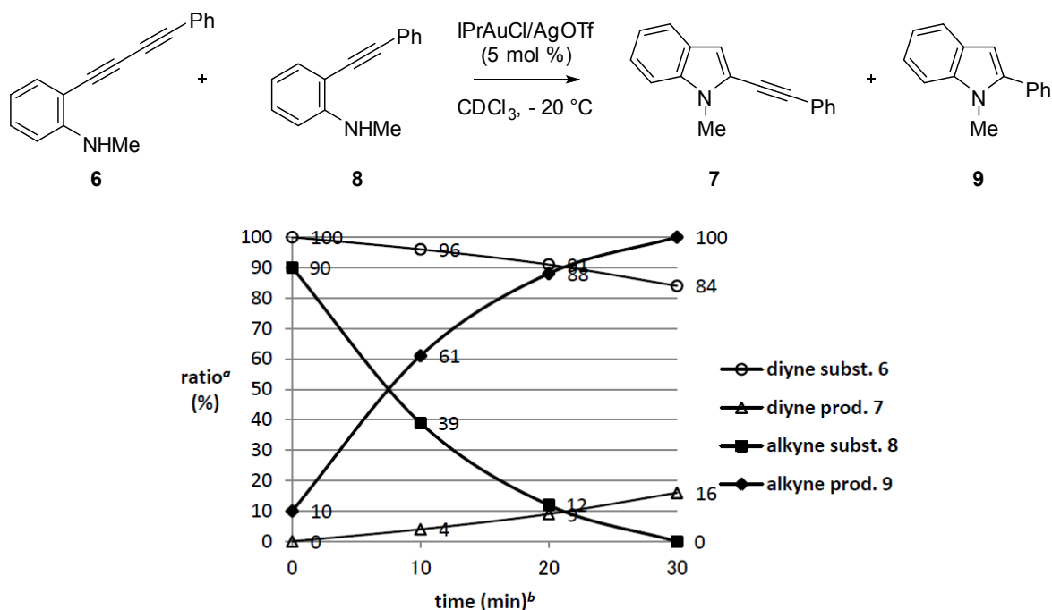
Scheme 3. NMR Analysis of Comparison of the Reactivities toward Indole Formation between Diynyl- and (Phenylethynyl)anilines
