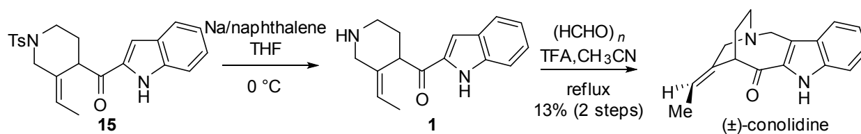
Scheme 7. Total Synthesis of ( \pm )-Conolidine
