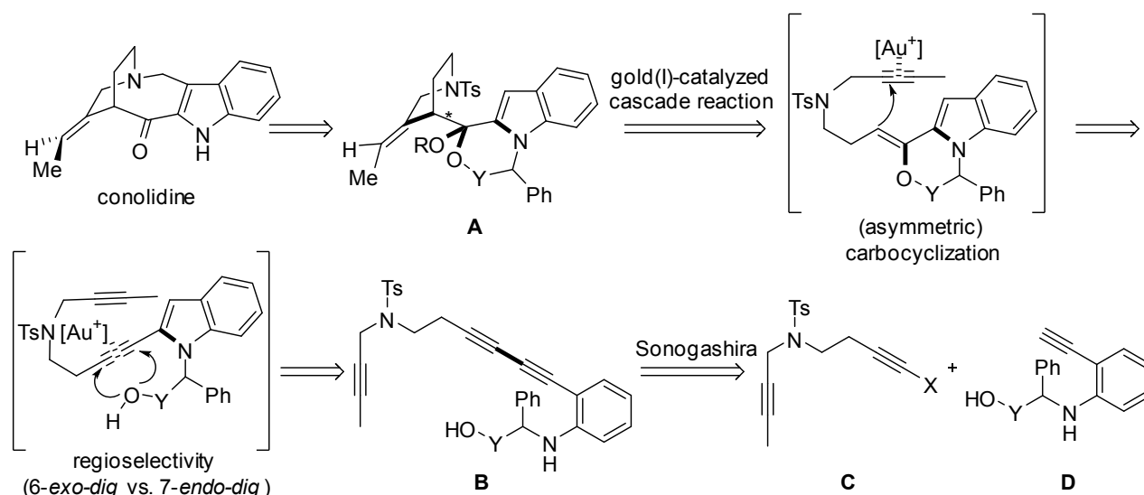
Scheme 9. The Author's Strategy (3-1): The First Strategy for the Total Synthesis of Conolidine by Cascade Cyclization of Conjugated Diyne
