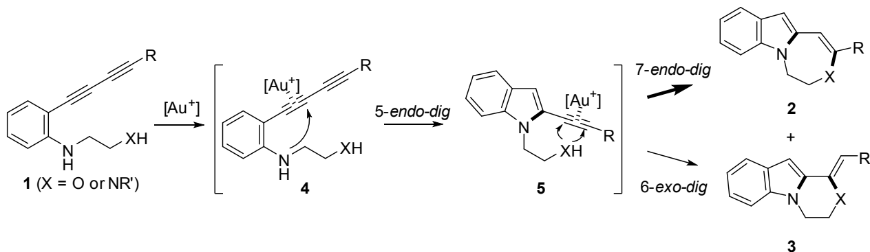
Scheme 1. Gold(I)-Catalyzed Intramolecular Consecutive Cyclization of a Conjugated Diyne
