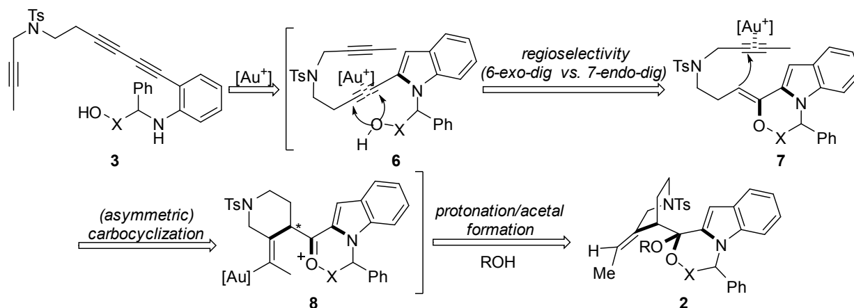
Scheme 2. Potential Regioselectivity Issues in Gold(I)-Catalyzed Cascade Reaction
