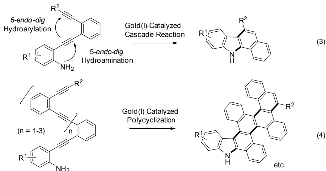
Scheme 4. Gold(I)-Catalyzed Cascade Cyclization Reaction of Polyyne-Type Anilines
