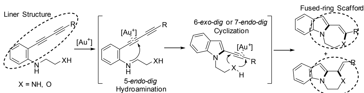
Scheme 7. The Author's Concept (2): Gold(I)-Catalyzed Addition Cascade of Conjugated Diynes
