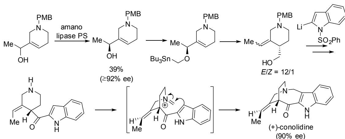
Scheme 8. Total Synthesis of (+)-Conolidine Reported by Bohn et al.
