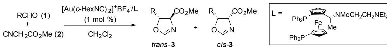
Scheme 2. Asymmetric Gold(I)-Catalyzed Aldol Reaction by Ito and Hayashi et al.
