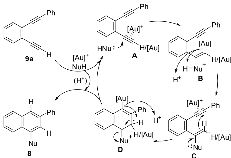
Scheme 5. A Plausible Catalytic Cycle
