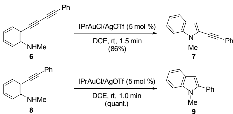
Scheme 2. Comparison of the Reactivities toward Indole Formation between Diynyl- and (Phenylethynyl)anilines
