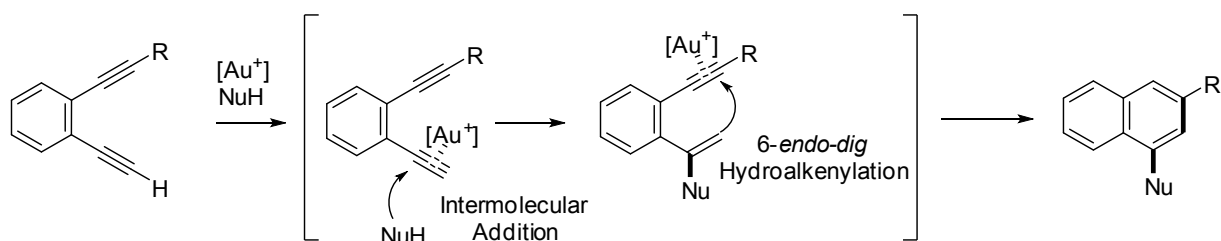
Scheme 5. The Author's Concept (1): Gold(I)-Catalyzed Addition Cascade of Dialkynylbenzenes Using External Nucleophiles
