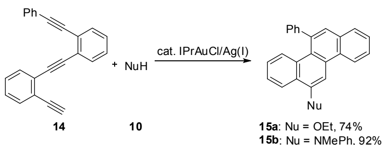
Scheme 11. Application to Consecutive Cyclization
