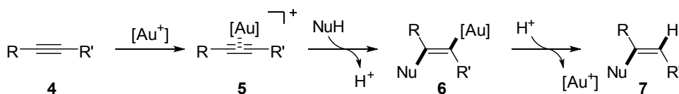
Scheme 3. Cationic Gold(I)-Catalyzed Nucleophilic Addition to Alkynes
