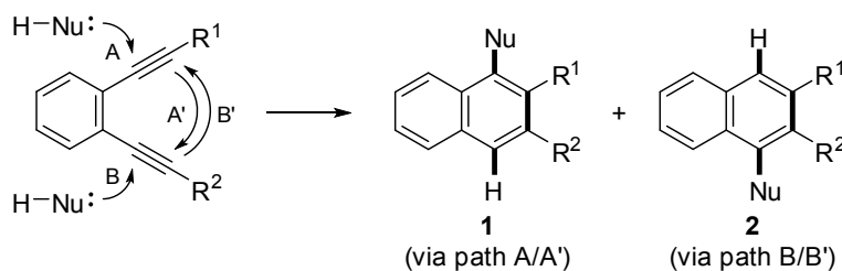
Scheme 2. The Regioselectivity Issue for Intermolecular Addition
