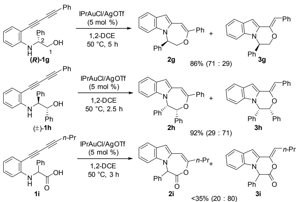
Scheme 4. Investigation of the Nucleophilic Moiety.
