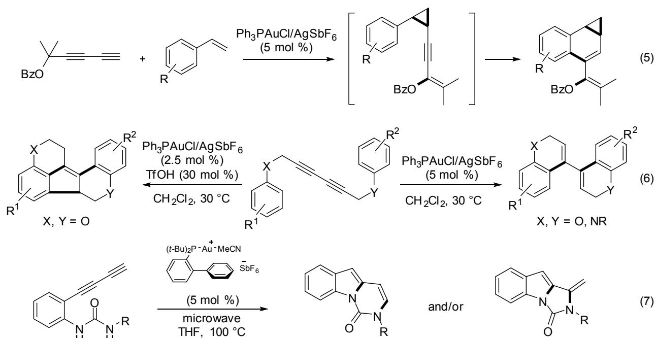
Scheme 6. Gold(I)-Catalyzed Reactions of Conjugated Diynes
