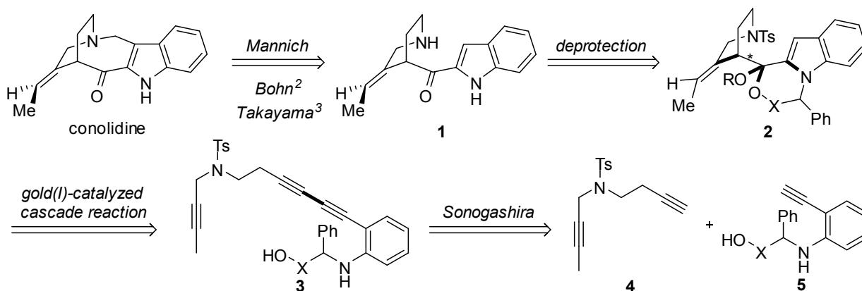
Scheme 1. The Author's Strategy (1): Gold(I)-Catalyzed Cascade Reaction of Conjugated Diynes
