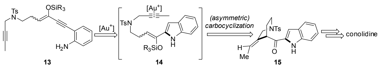
Scheme 5. The Author's Strategy (2): Gold(I)-Catalyzed Cascade Cyclization of Conjugated Enyne-type Silyl Enol Ether
