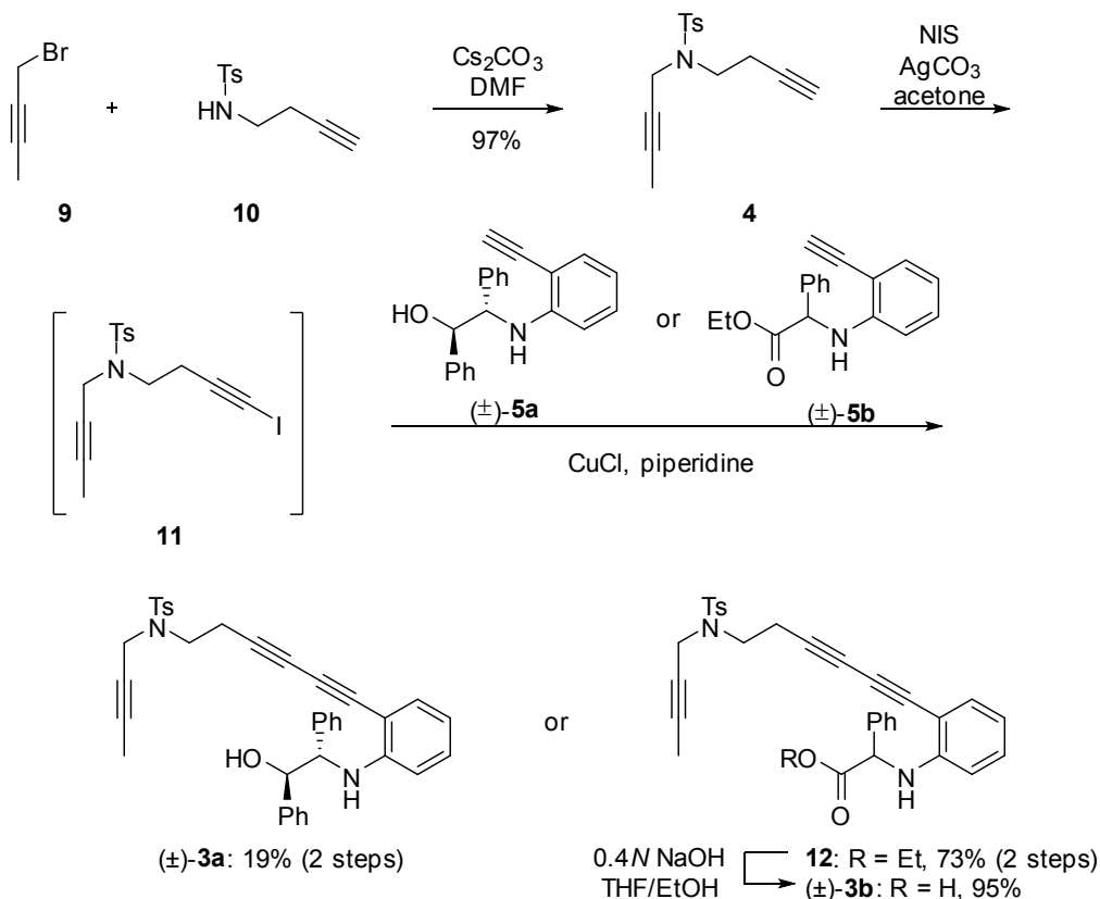
Scheme 3. Preparation of the conjugated diynes (±)-3a and (±)-3b
