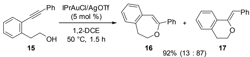
Scheme 6. Reaction of the Benzene Congener 15
