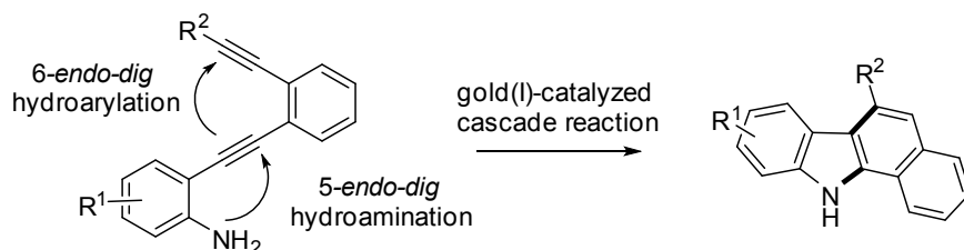
Scheme 1. Gold(I)-Catalyzed Cascade Cyclization Reaction of Polyyne-Type Anilines
