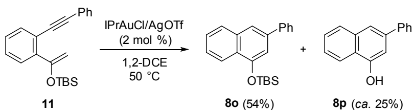
Scheme 6. Reaction of the Silyl Enol Ether 11
