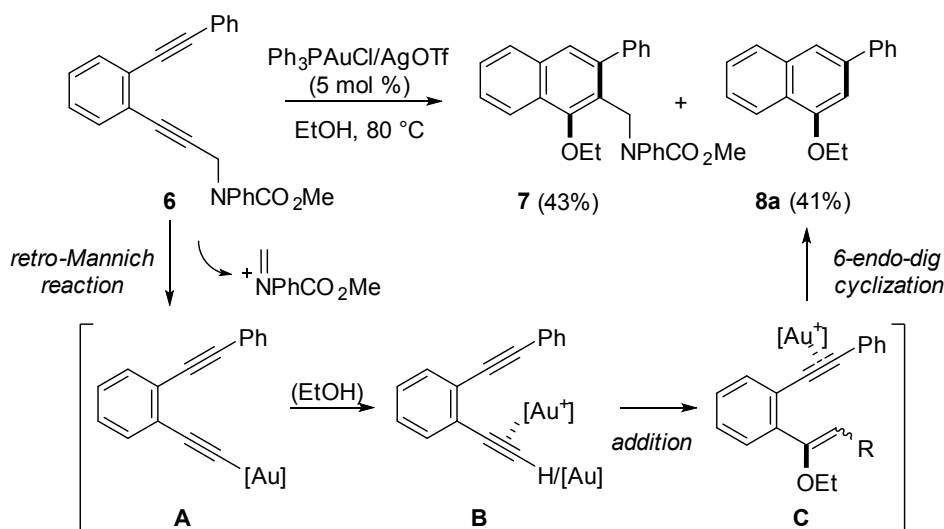
Scheme 4. Unexpected Regioselective Formation of 1-Ethoxy-3-phenylnaphthalenes
