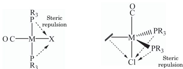
Figure 2.3: Illustration of steric repulsion.
