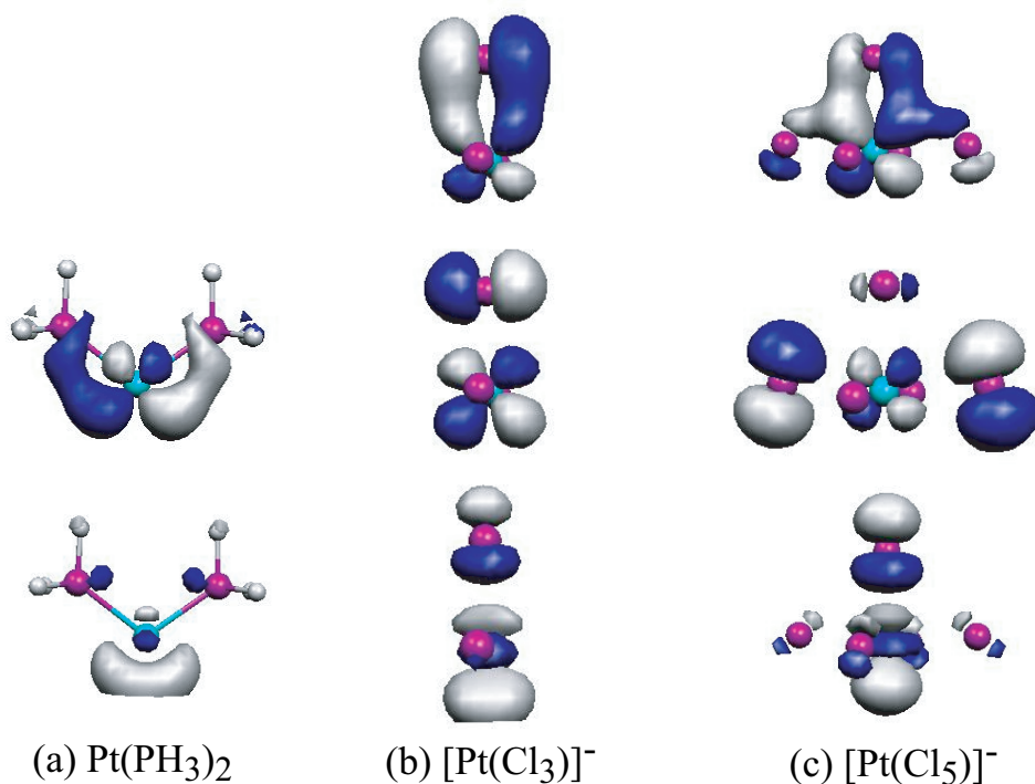
Figure 1.10: d_{\pi} - and d_{\sigma} -type orbitals of (a) Pt(PH 3 ) 2 , (b) [PtCl 3 ] − , and (c) [PtCl 5 ] − .
